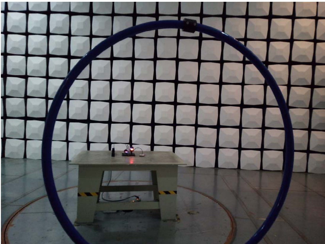
Radiated Emission Below 30M View
