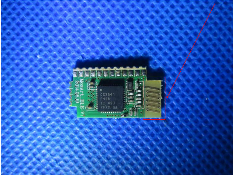
BT4.0 Antenna
