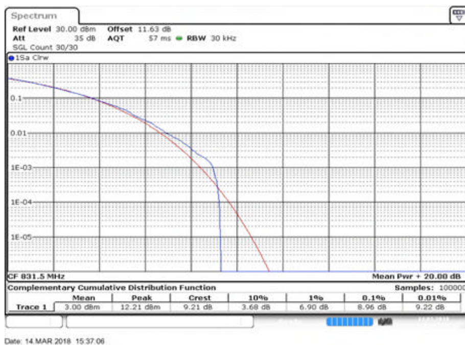
Peak-Average Ratio Plot(5MHz BW,16QAM,Band 26-mid Channel)
