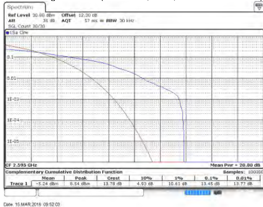
Peak-Average Ratio Plot(10MHz BW,16QAM,Band 41-mid Channel)
