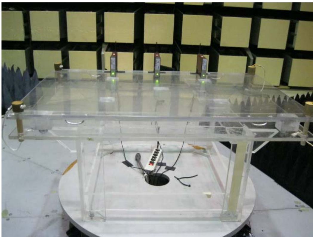
Radiated Emissions; Spurious to 18 GHz; Front
