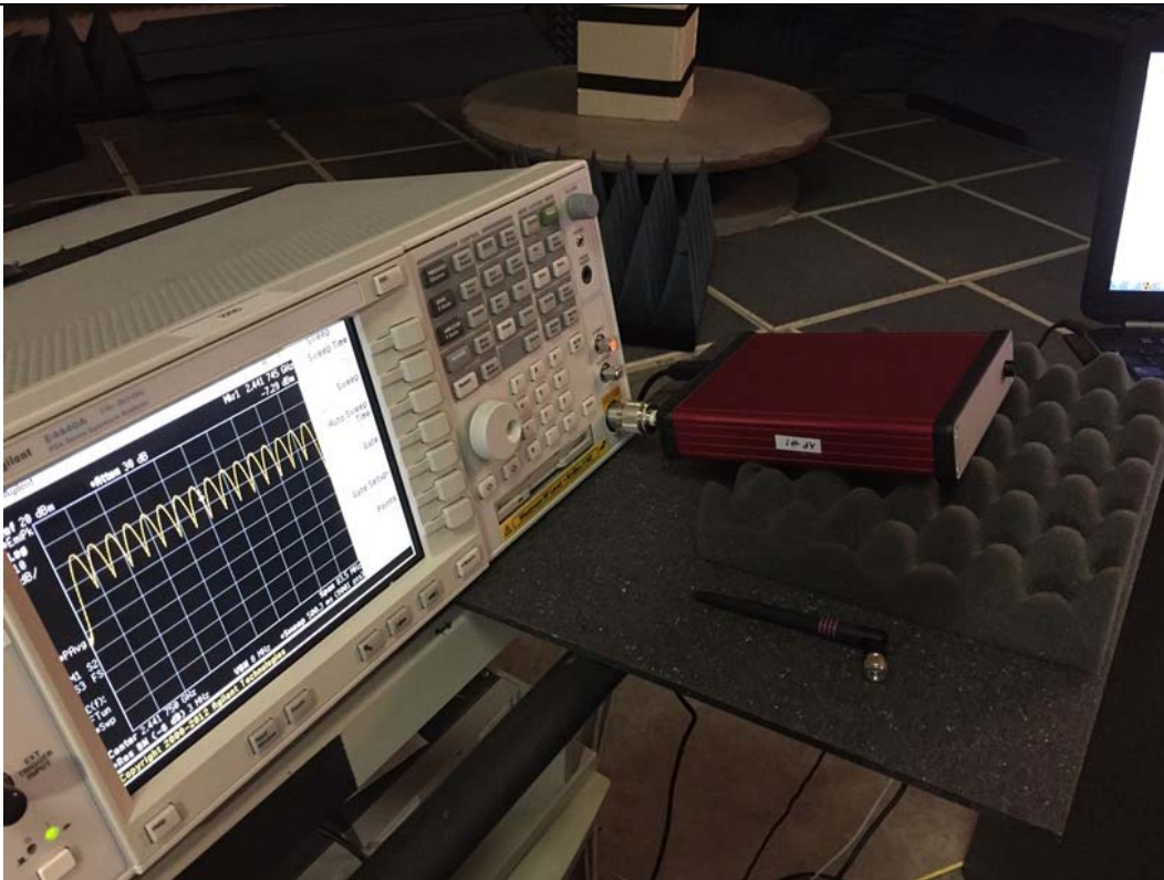
Conducted Antenna Port Measurements; Power, Bandwidth, Band Edge
