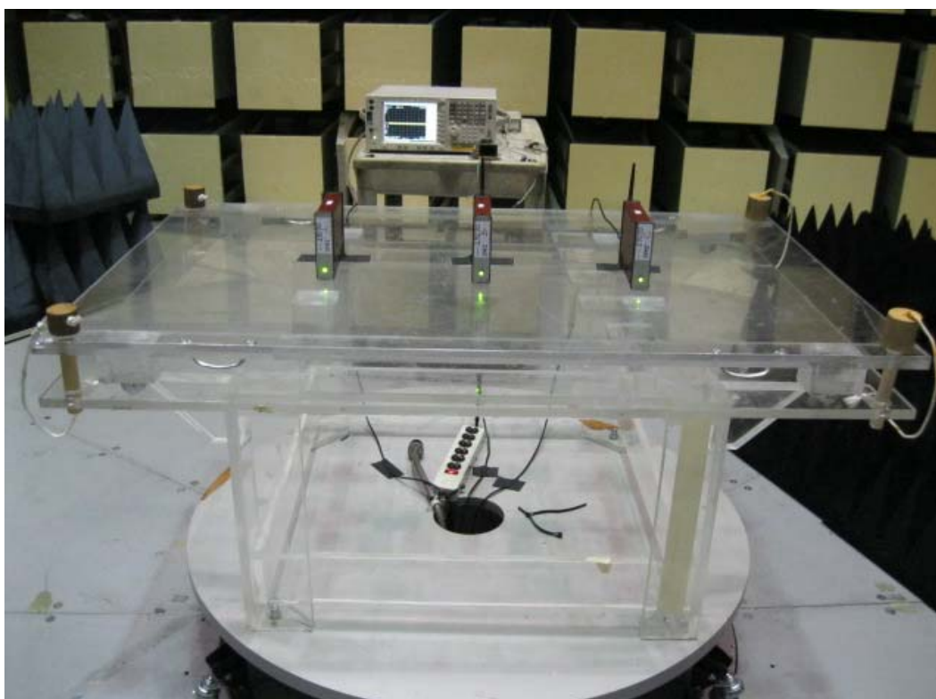
Radiated Emissions; Spurious to 25 GHz; Back
