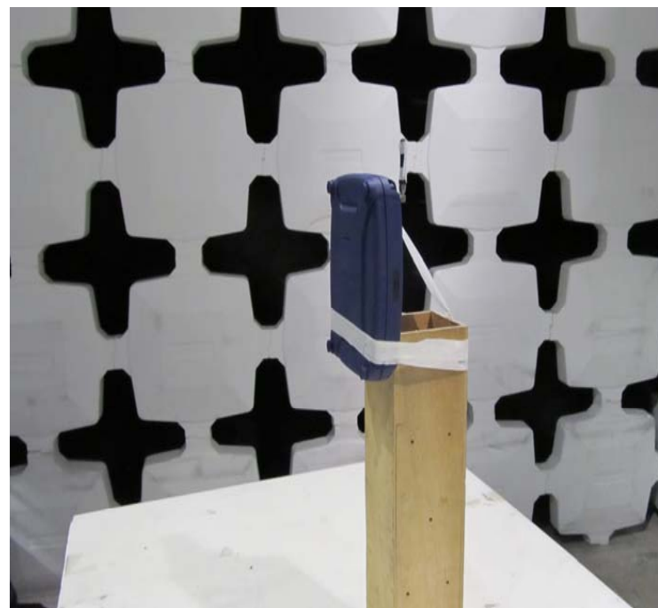
Radiated emissions test set up. General view.
