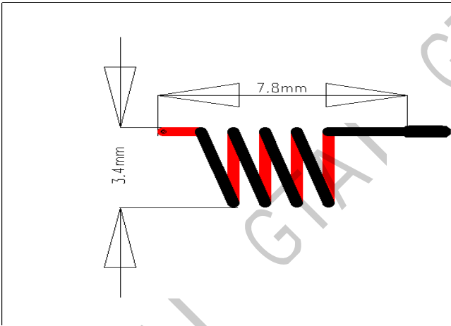
Antenna Photo & Length (mm). 板载天线
