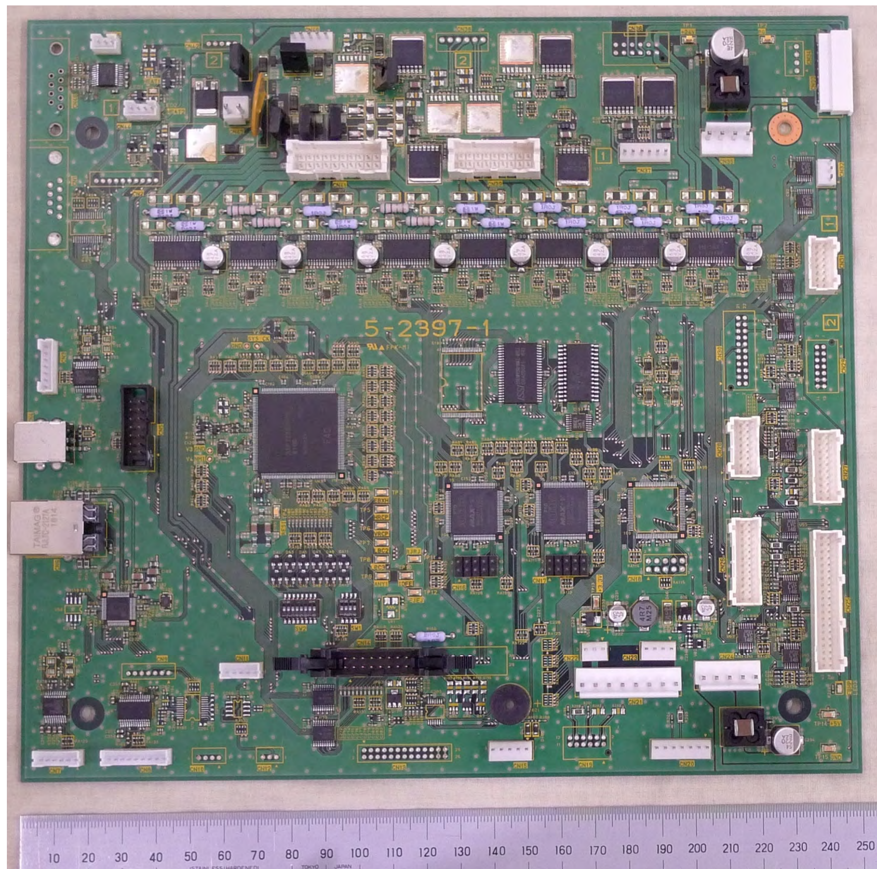
(a) Main Controller Board – Top side
