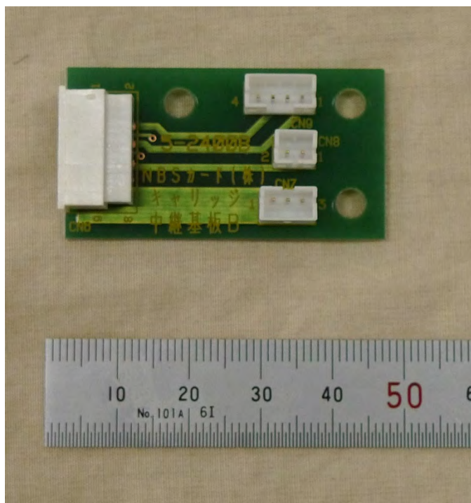
(i) Carriage junction board B – Top side
