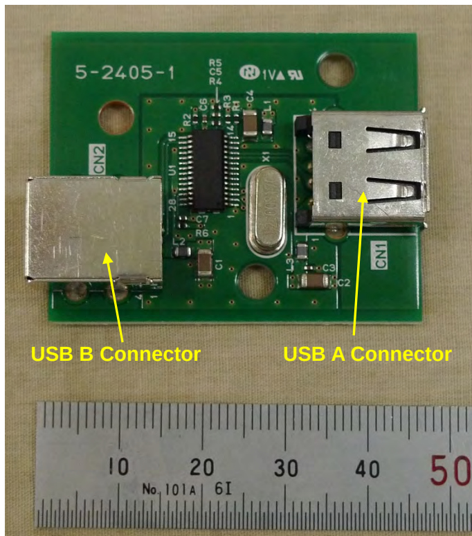
(b) USB - HUB board – Top side
