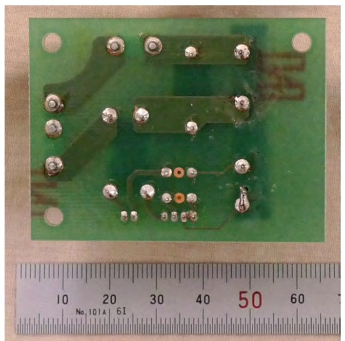
(c) SSR board – Bottom side
