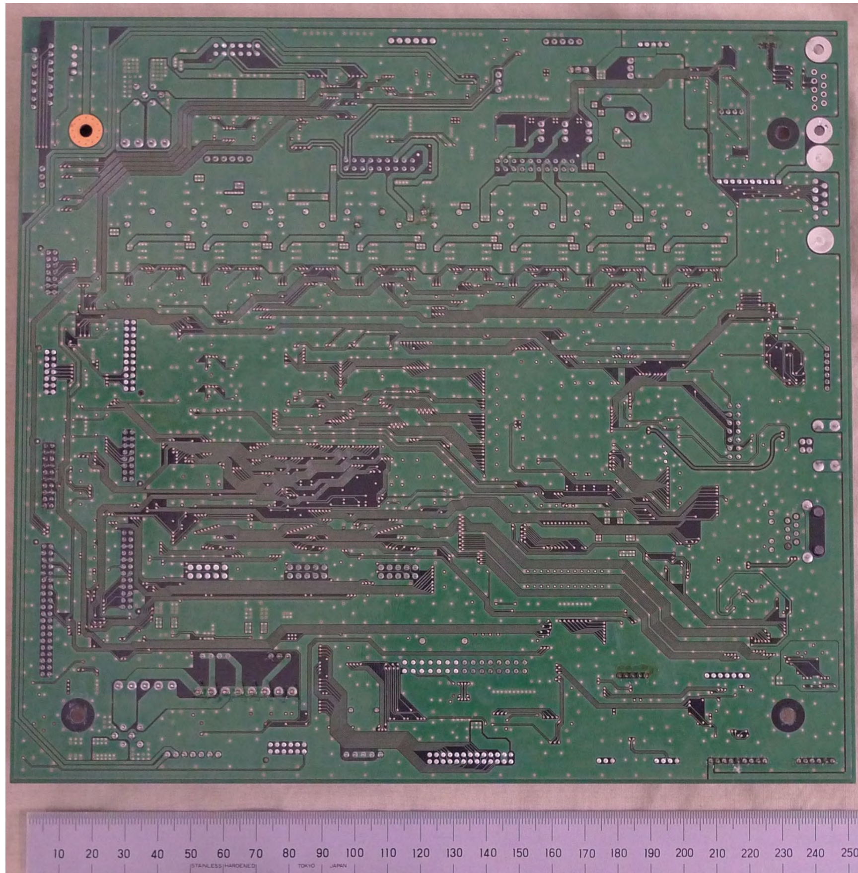
(a) Main Controller Board – Bottom side
