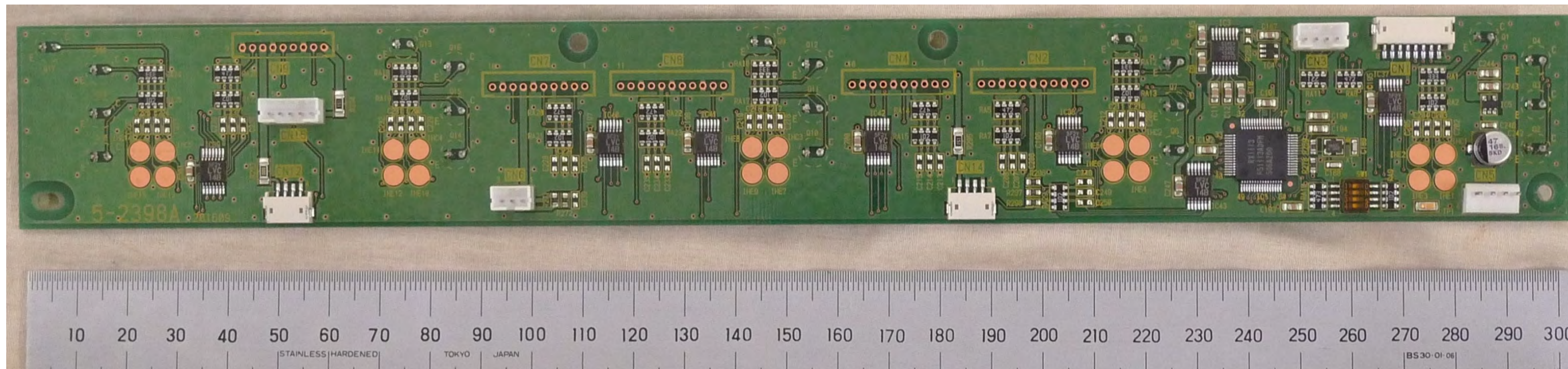
(f) Input Hopper board A – Bottom side
