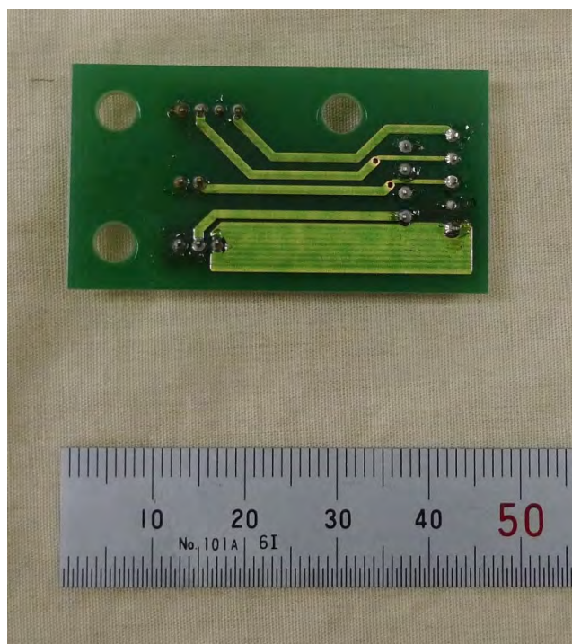
(i) Carriage junction board B – Bottom side
