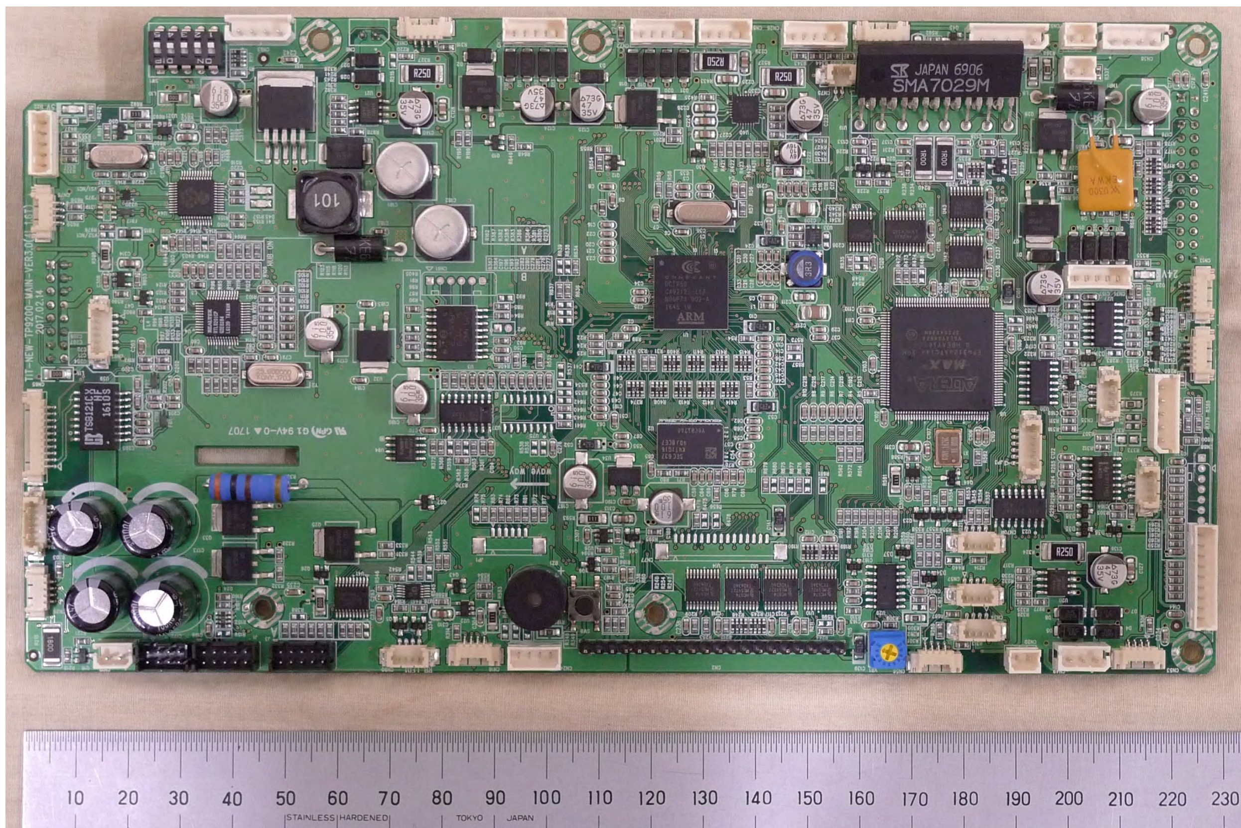
(j) Main Board – Top side
