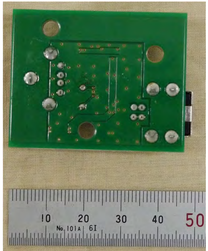
(b) USB - HUB board – Bottom side
