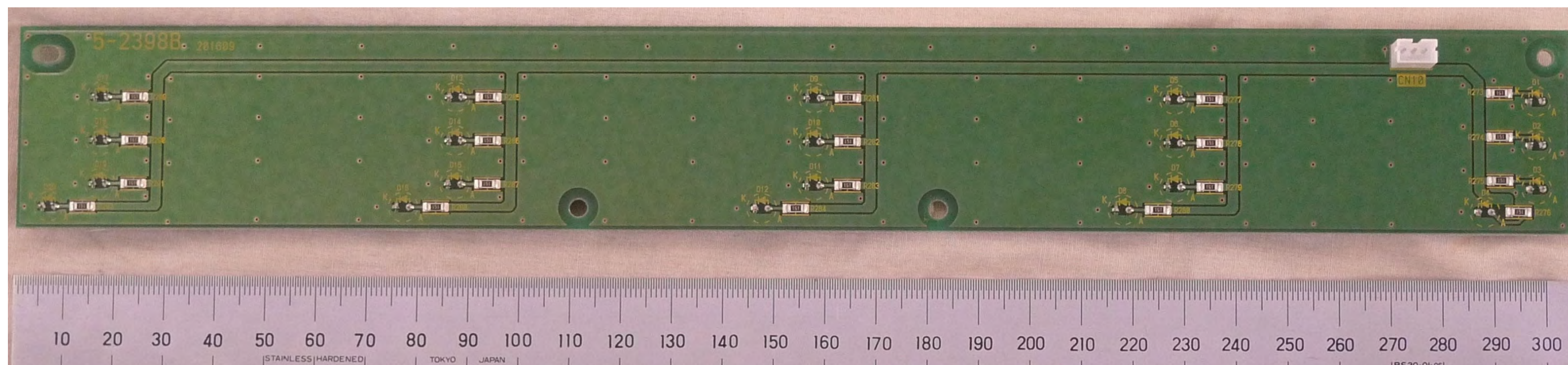
(g) Input Hopper board B – Top side
