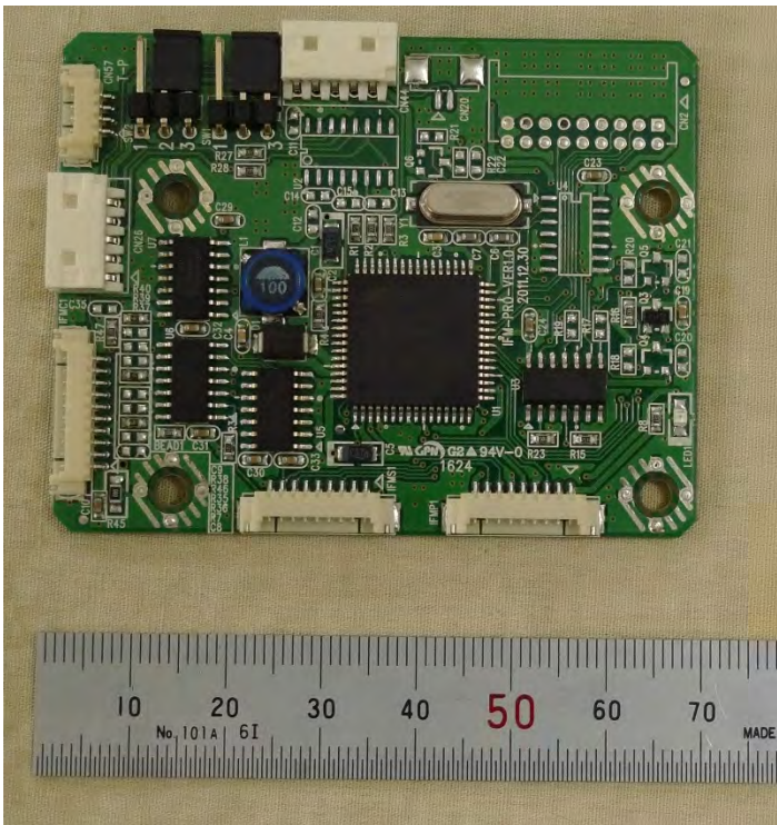
(n) IFM Board–Top side
