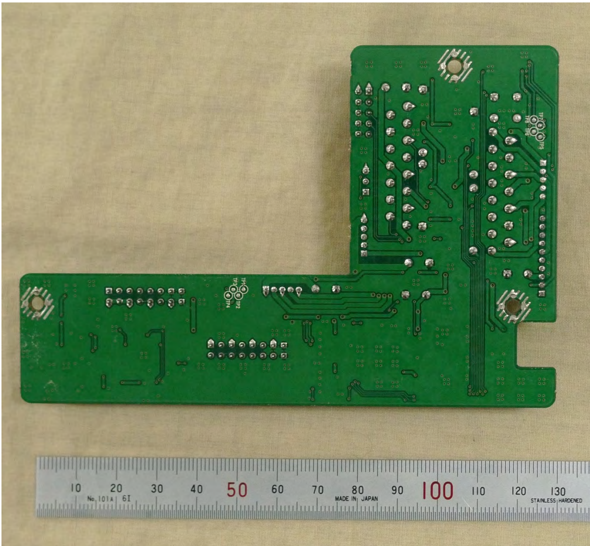
(o) Side change Board – Bottom side
