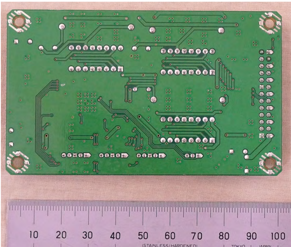
(p) MSRD Board – Bottom side
