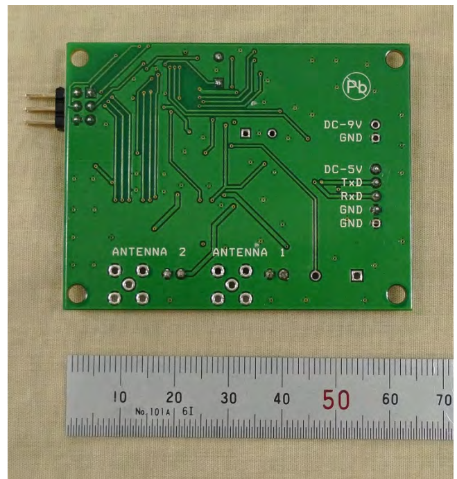
(l) RF READER Board –Bottom side
