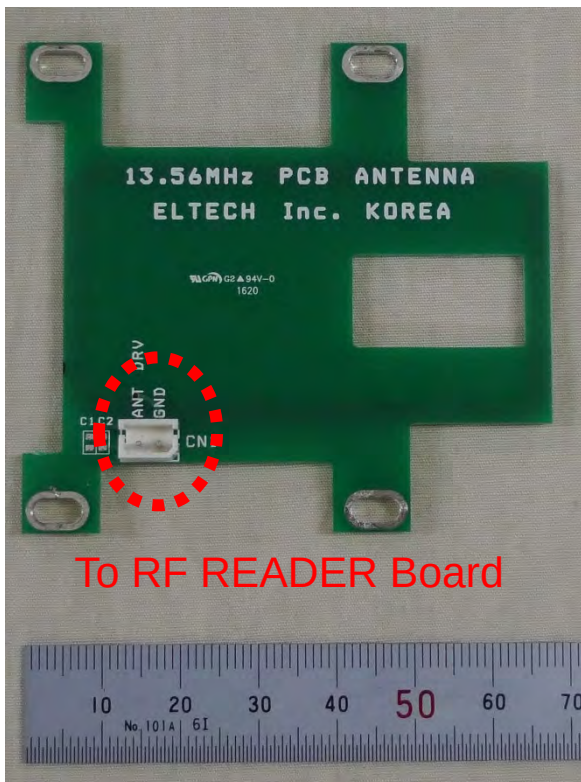
(m) ANT Board–Top side
