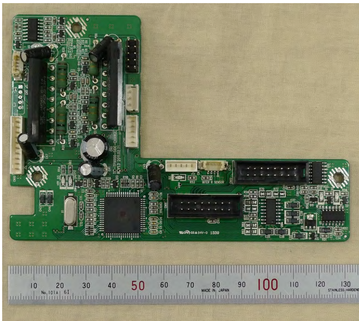
(o) Side change Board—Top side
