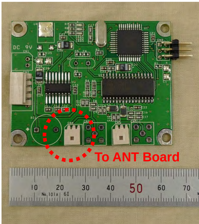
(l) RF READER Board – Top side
