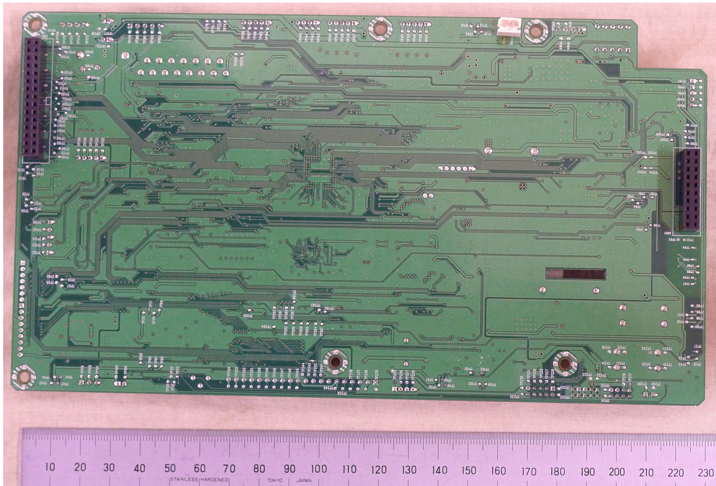
(j) Main Board – Bottom side
