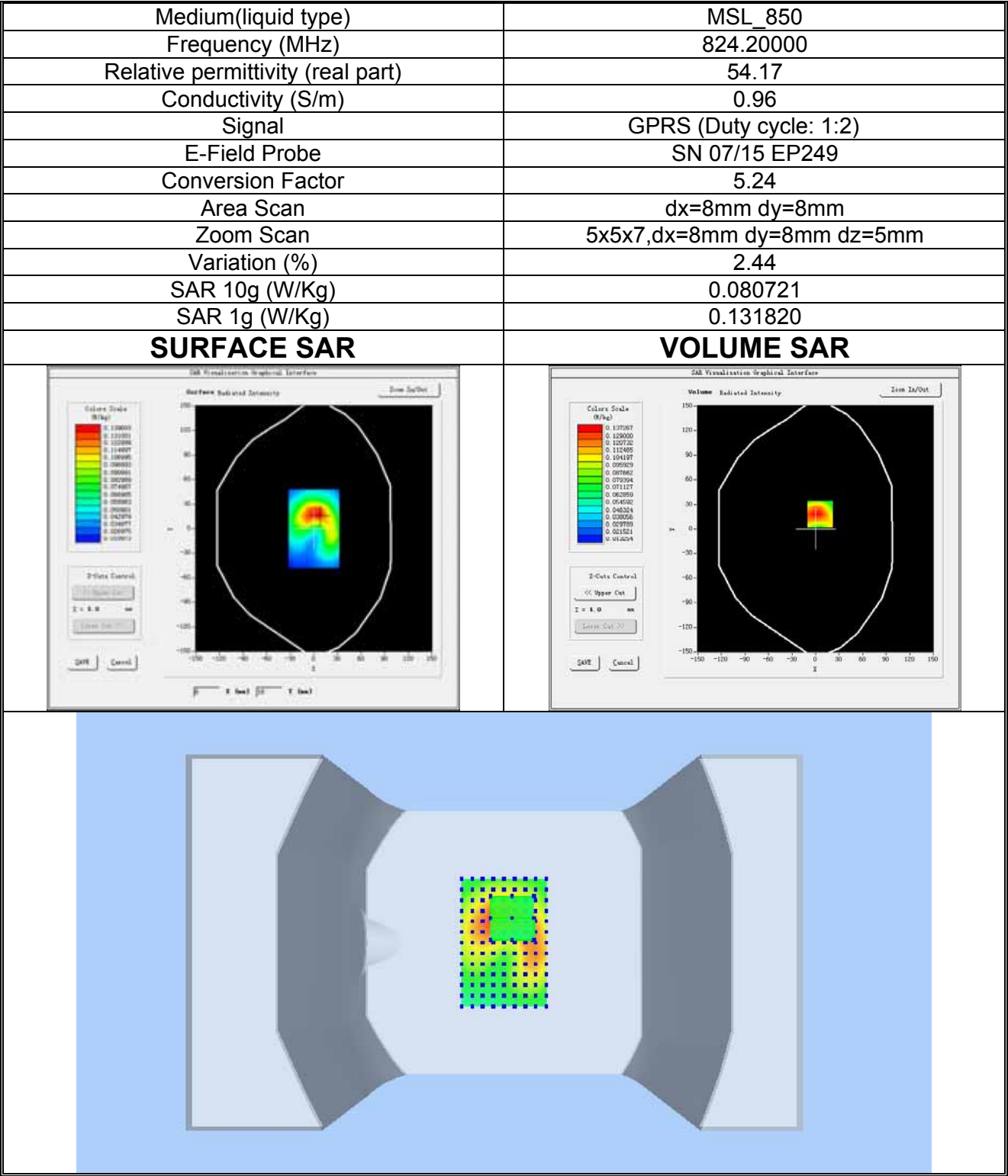
Plot 8: GPRS850MHz, Low channel(Body-worn, Bottom edge) Product Description: Mobile Phone Test Date: 2018-06-07
