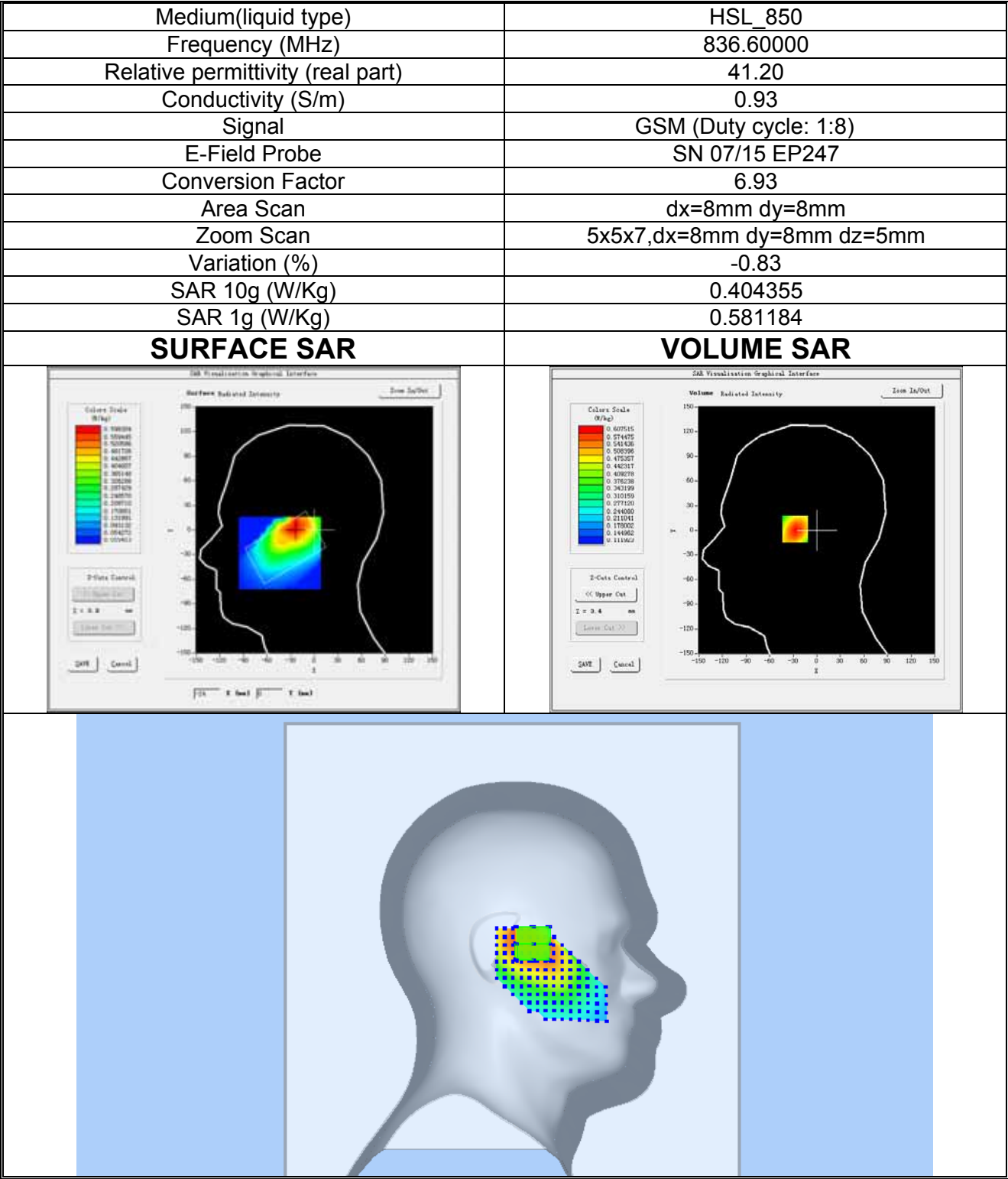
Plot 3: GSM850MHz, Mid channel (Left Head , Cheek) Product Description: Mobile Phone Test Date:2018-09-13
