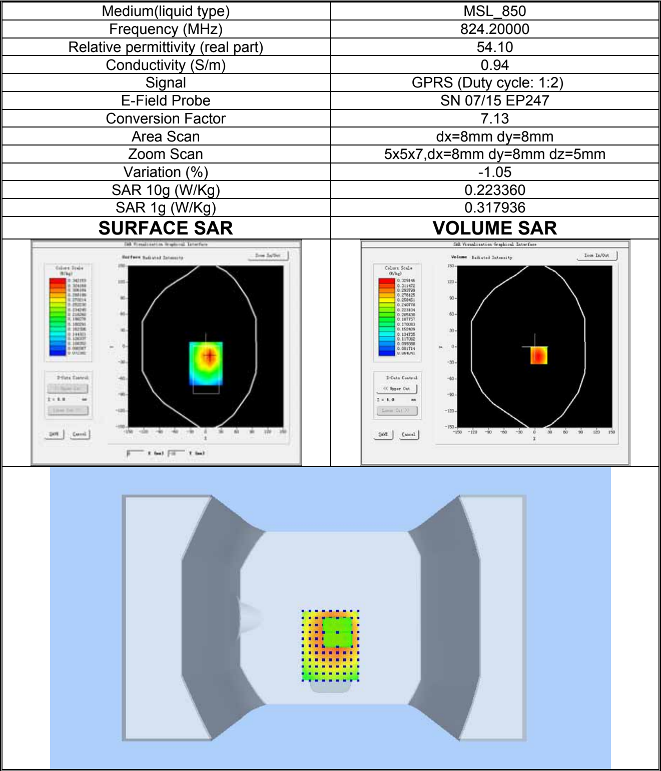
Plot 5: GPRS850MHz, Low channel(Body-worn, Front Surface) Product Description: Mobile Phone Test Date: 2018-09-13
