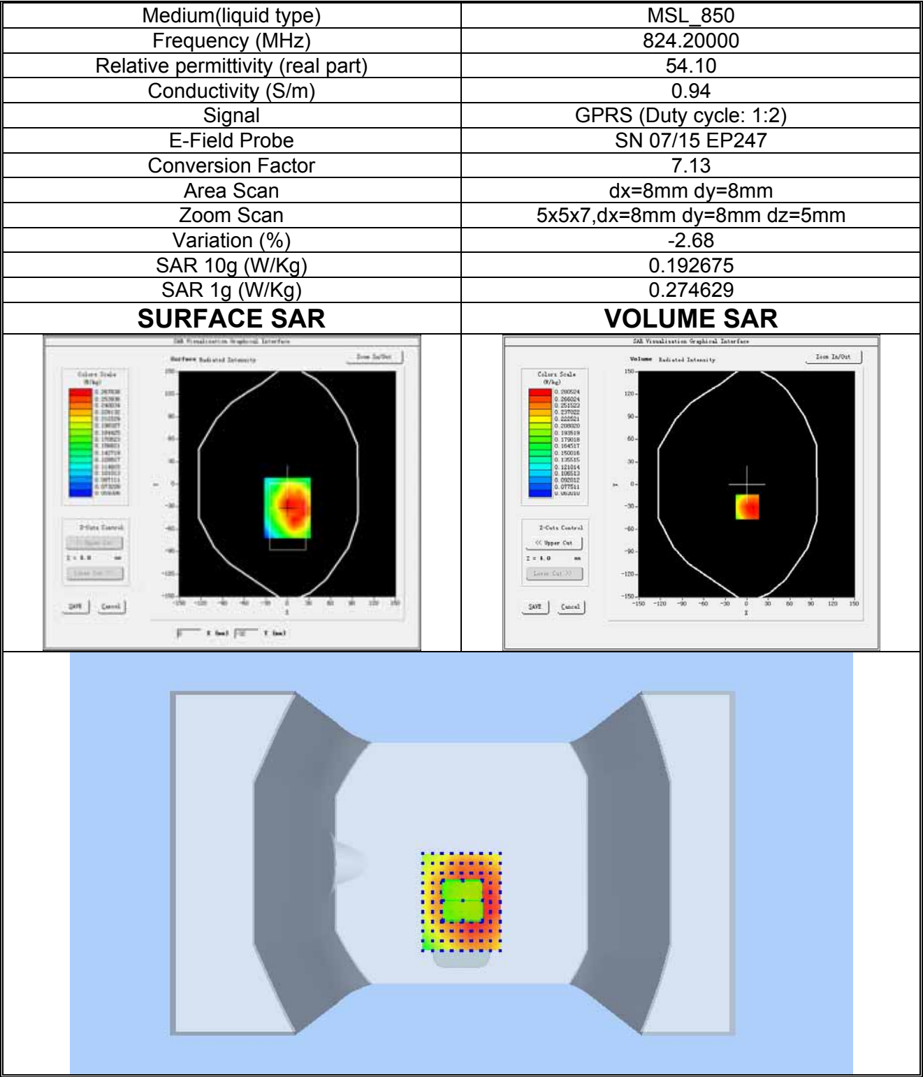
Plot 6: GPRS850MHz, Low channel(Body-worn, Back Surface) Product Description: Mobile Phone Test Date: 2018-09-13
