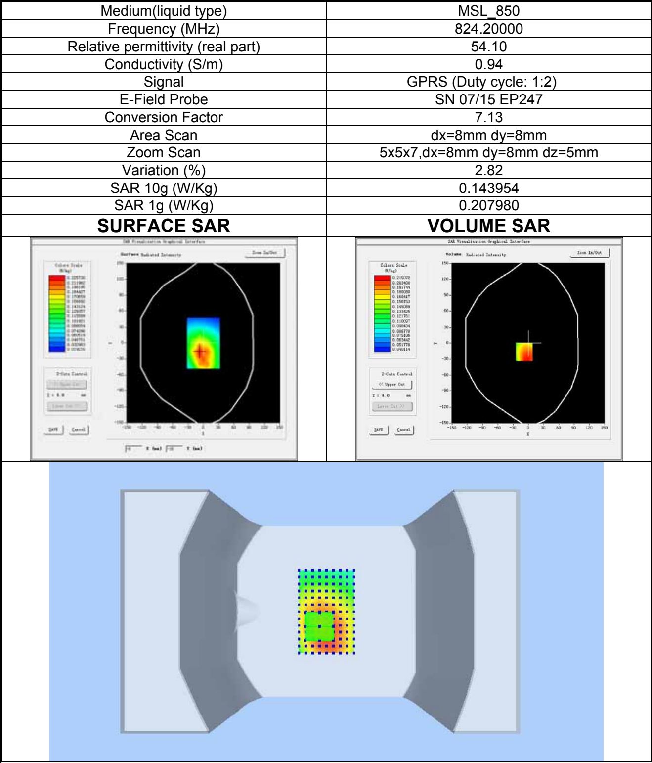
Plot 7: GPRS850MHz, Low channel(Body-worn, Right edge) Product Description: Mobile Phone Test Date: 2018-09-13
