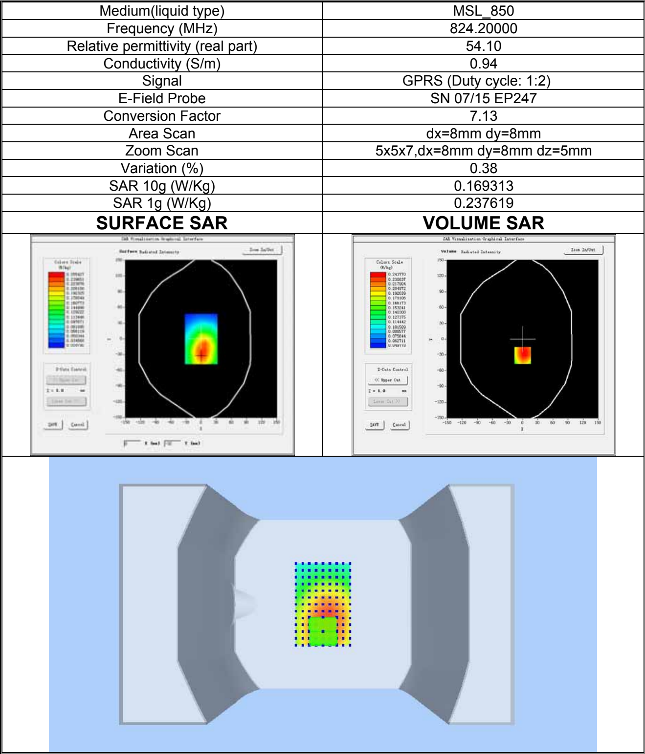
Plot 8: GPRS850MHz, Low channel(Body-worn, Left edge) Product Description: Mobile Phone Test Date: 2018-09-13
