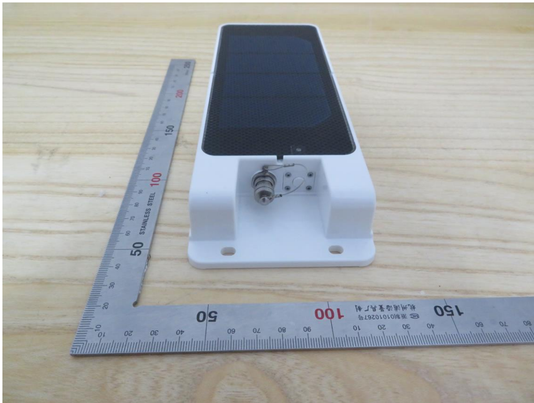
Back View of EUT- TT603-LM0Q-GL
