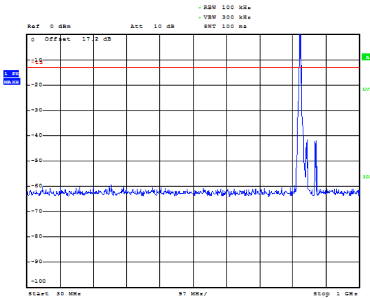
WCDMA Band V CH-Low 30MHz ~ 1GHz
