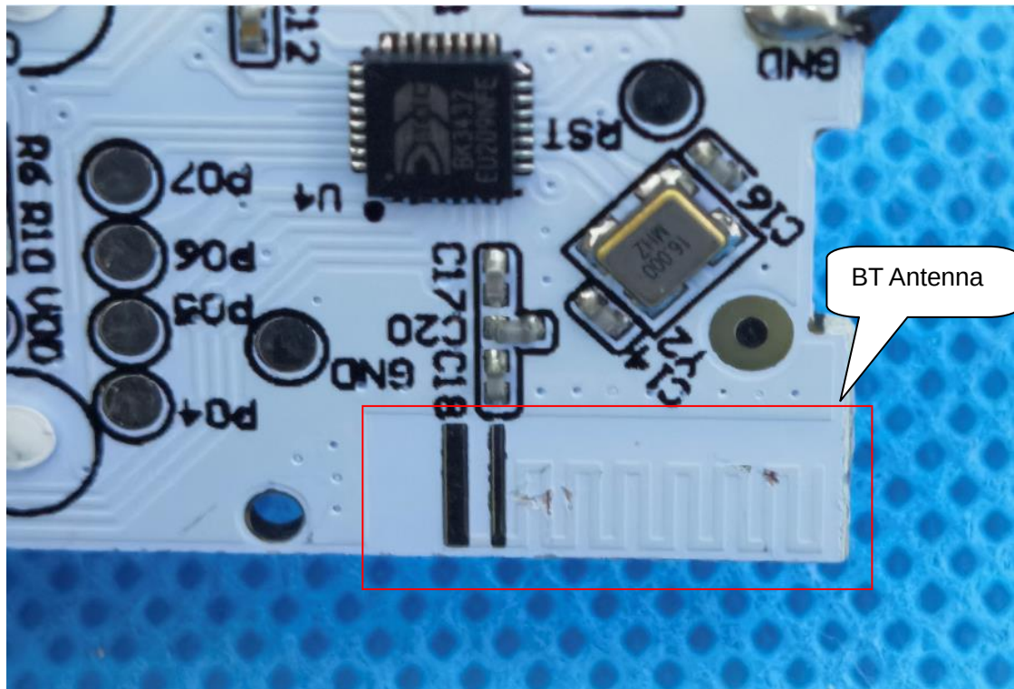
INTERNAL VIEW OF EUT (FIGURE 6)
