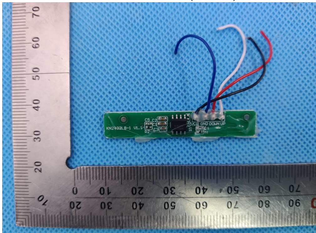
INTERNAL VIEW OF EUT (FIGURE 7)
