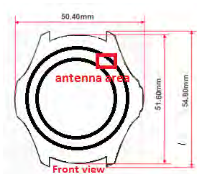
Fig.9 Antenna location
