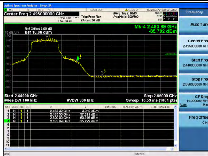
11N20SISO_Ant1_High_2462
