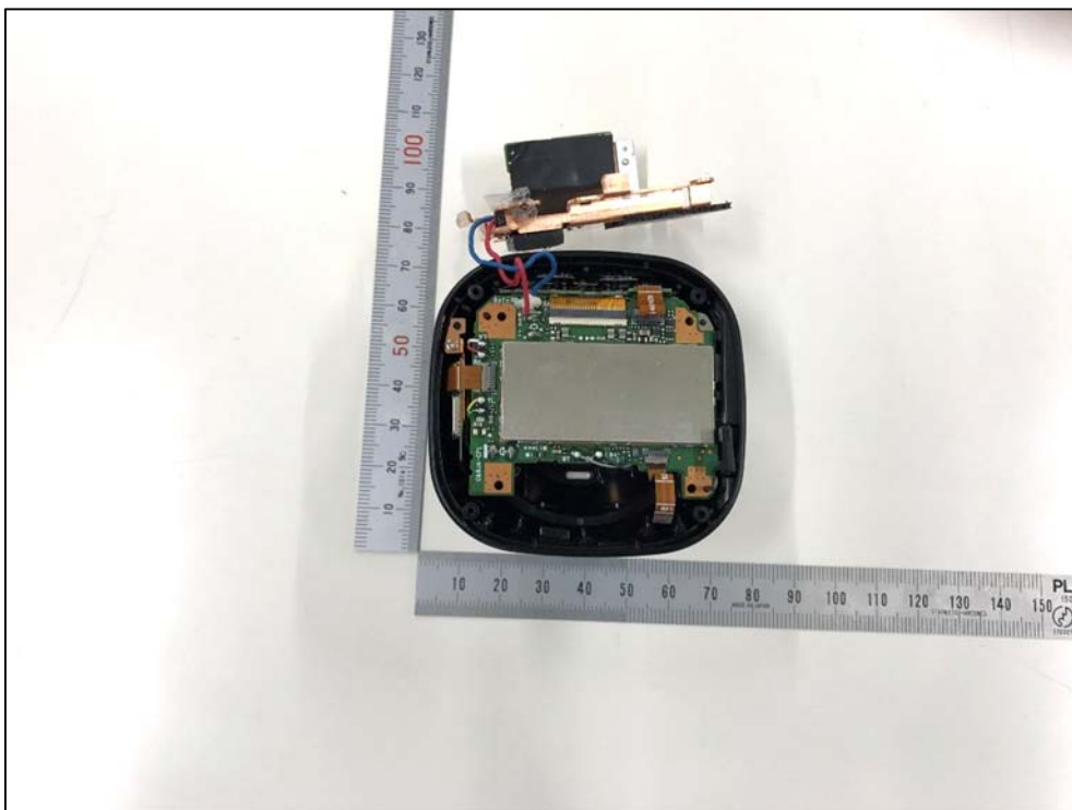
Heatsink removed
