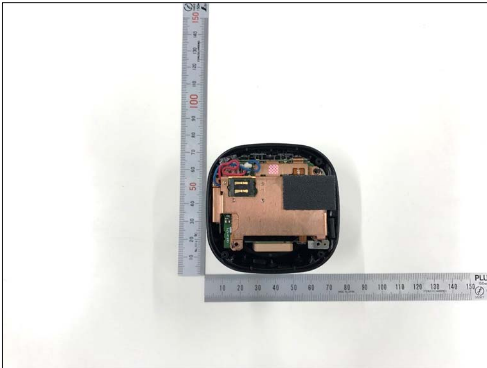
Cover removed
