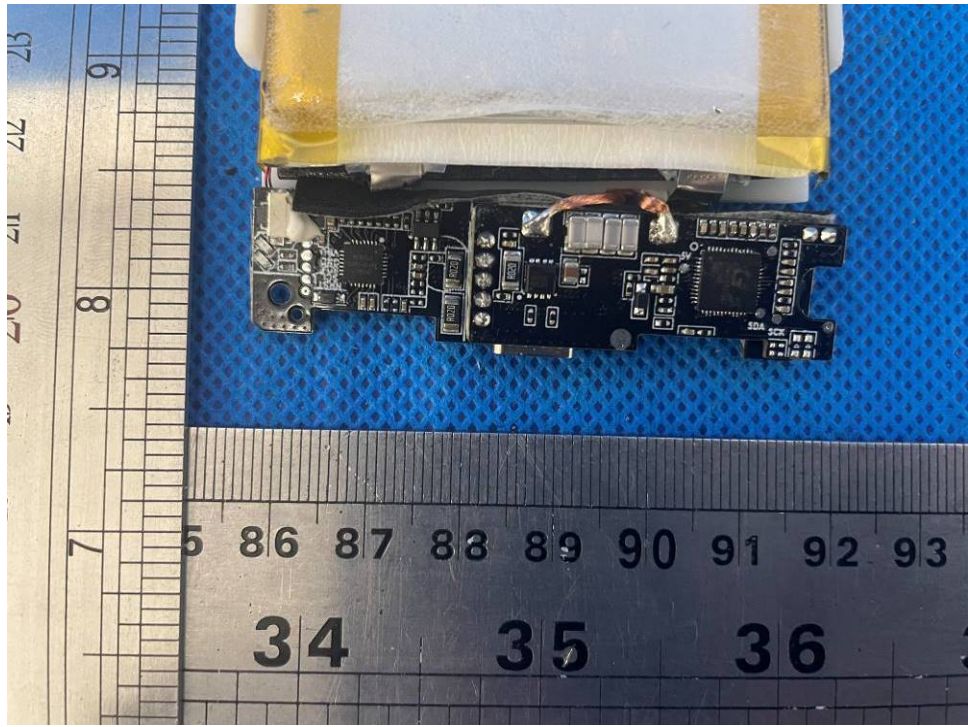
Figure 8 PCB view
