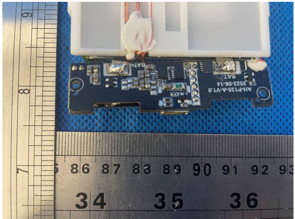
Figure 7 PCB view 1
