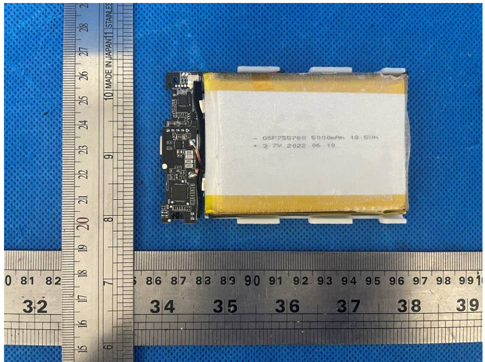
Figure 6 Internal view 3
