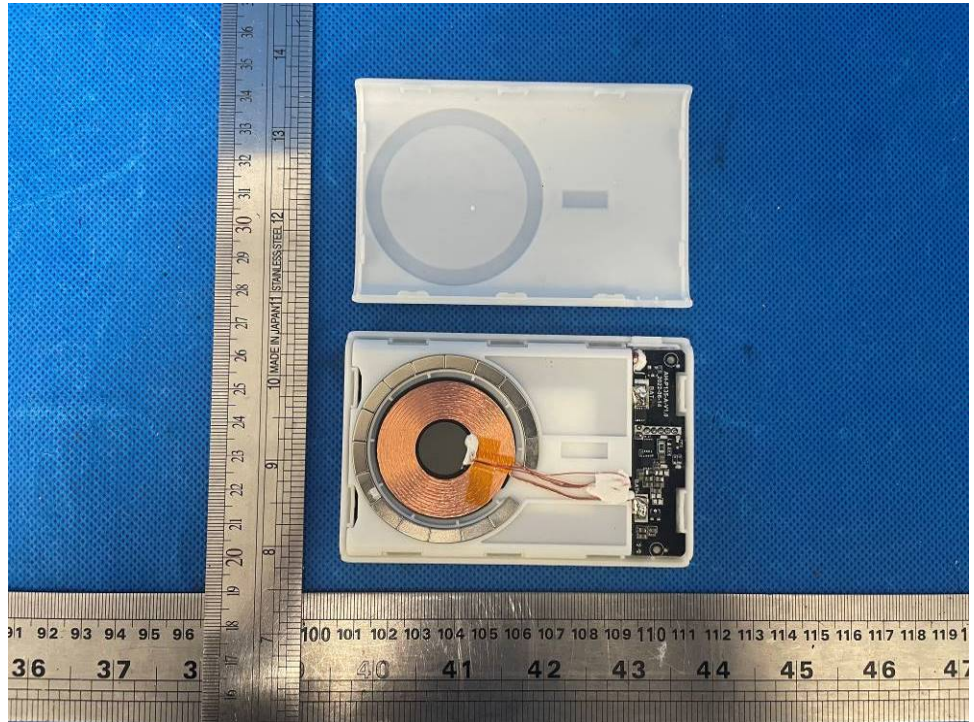
Figure 4 Internal view 1
