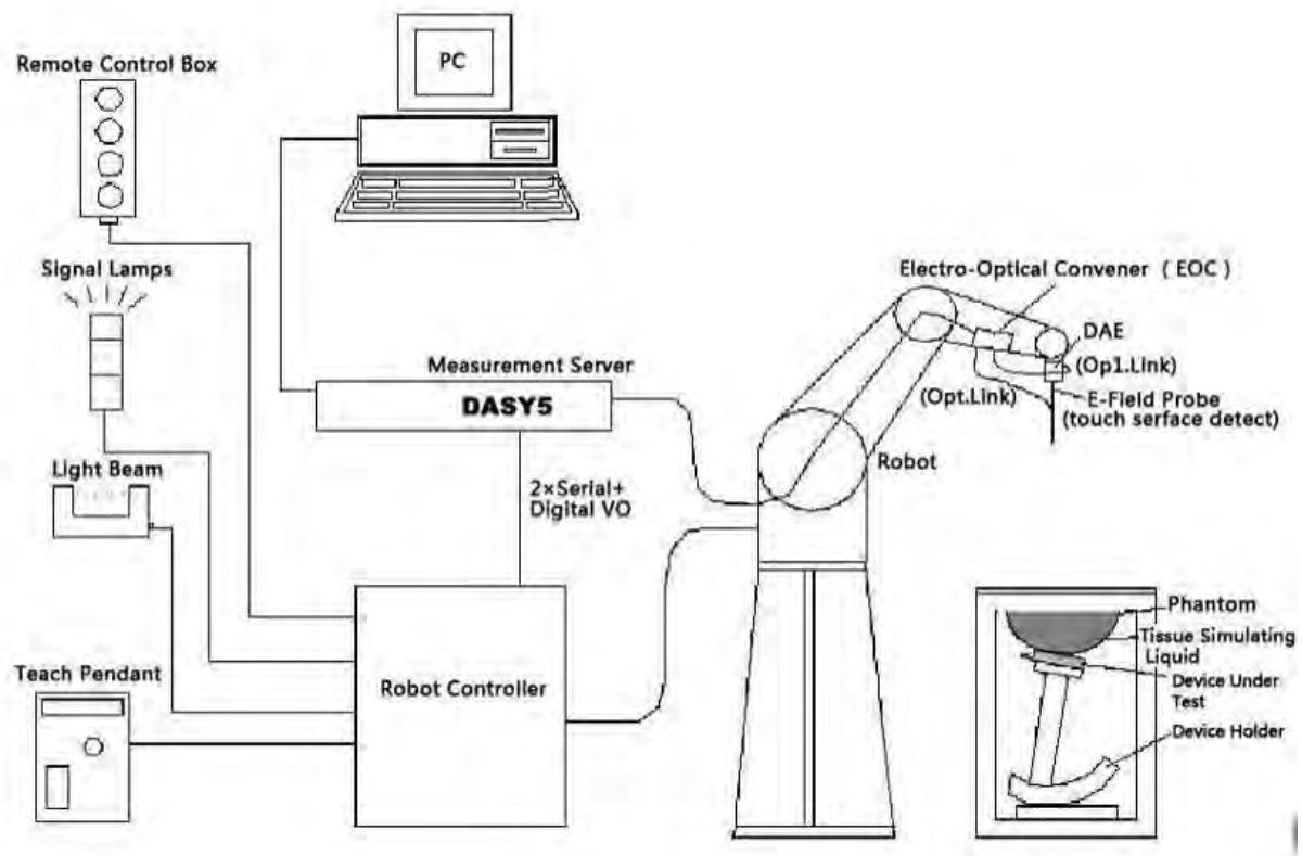
Picture 1. SAR Lab Test Measurement Set-up
