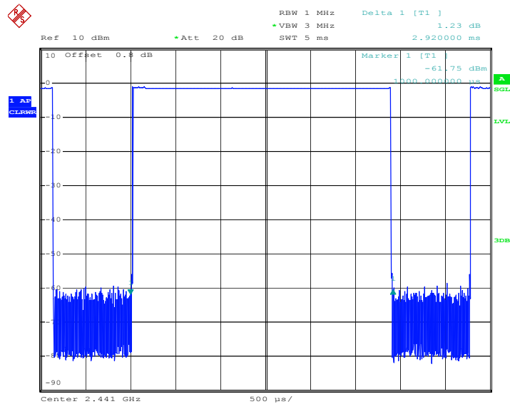
DH5 time slot (GFSK, Middle, Channels)
