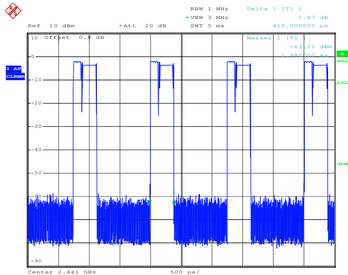
2DH1 time slot (4QPSK, Middle, Channels)
