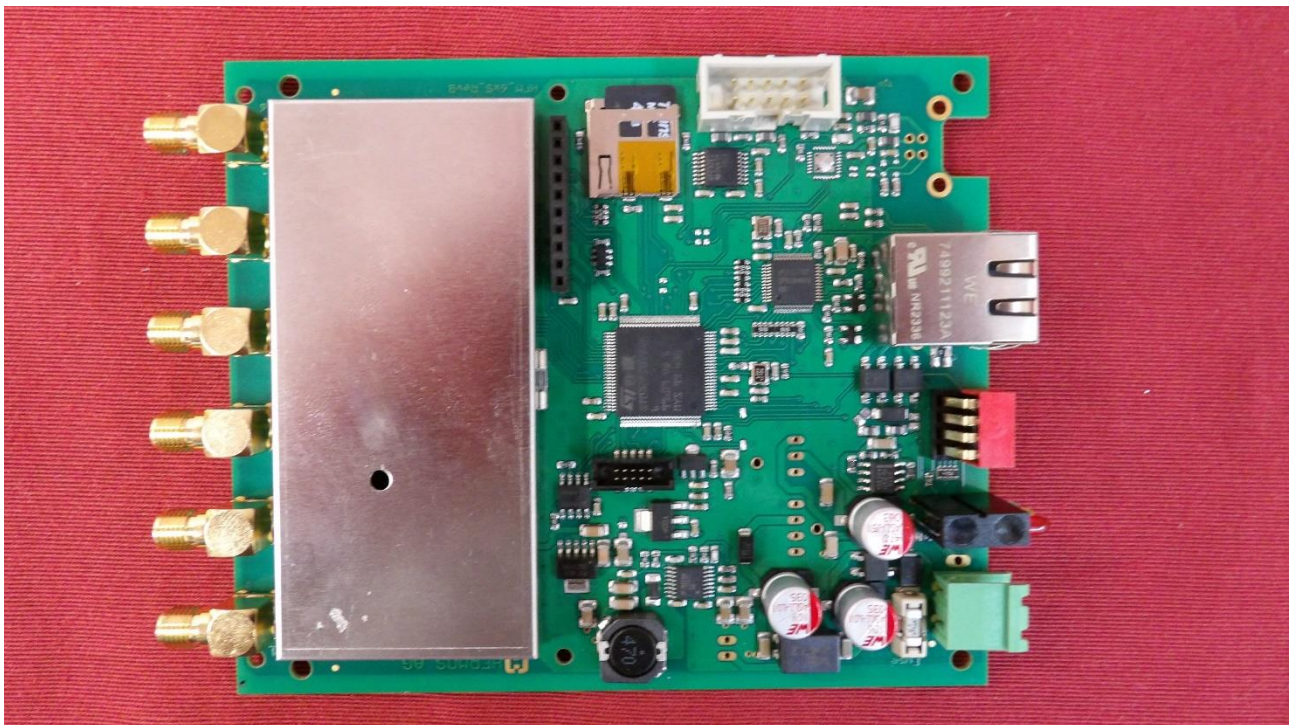
Picture 2: Top view of reading unit PCB, with shielding
