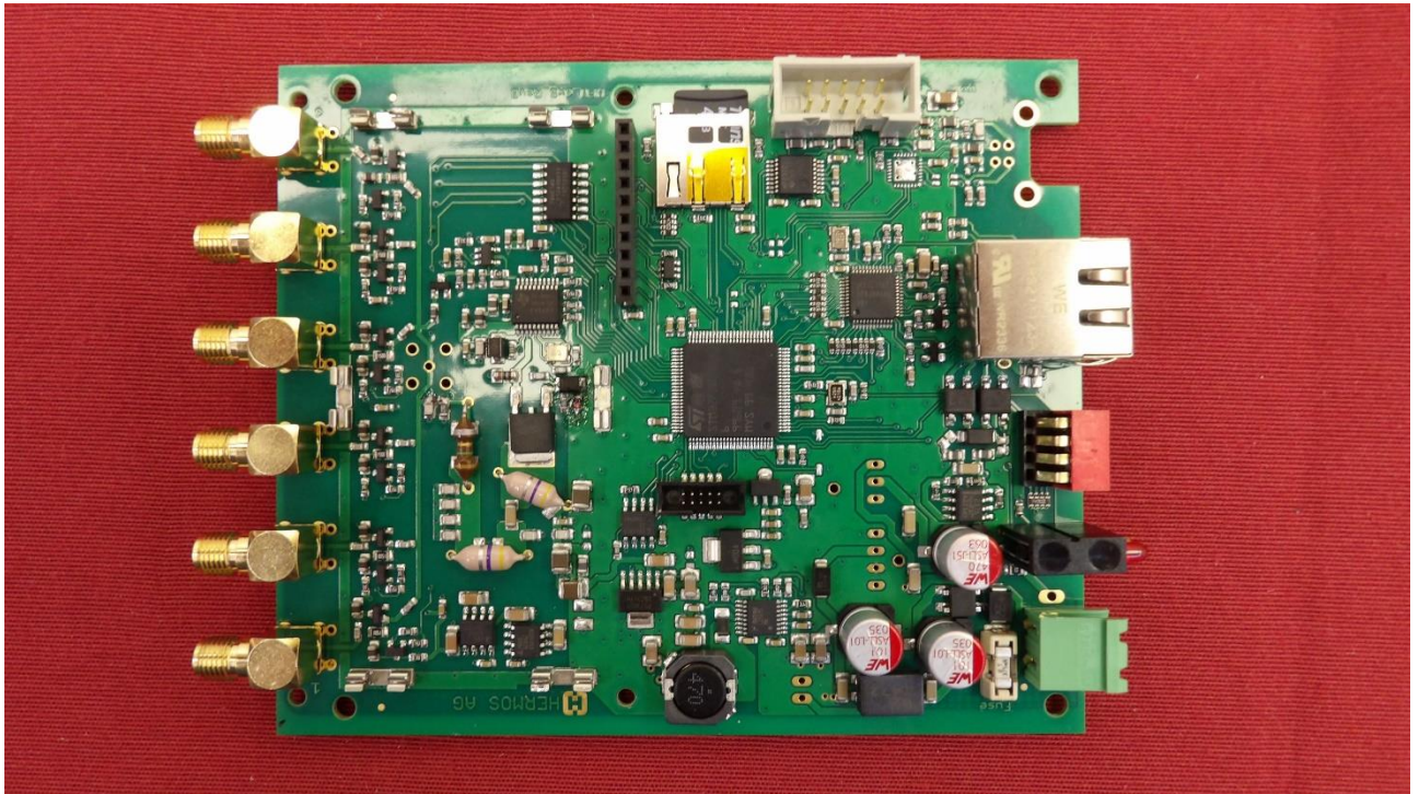
Picture 3: Top view of reading unit PCB, without shielding
