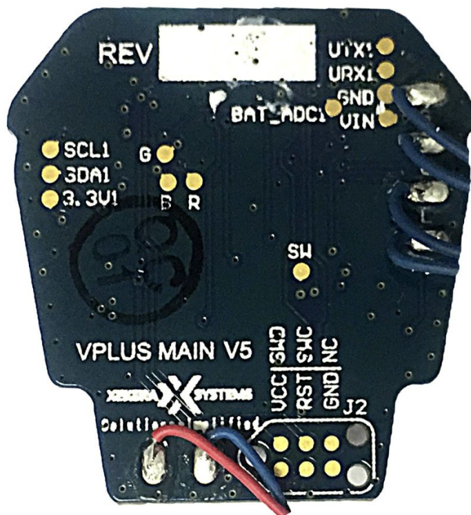
VPro+ Main Board: (BOTTOM VIEW, NO COMPONENTS)
