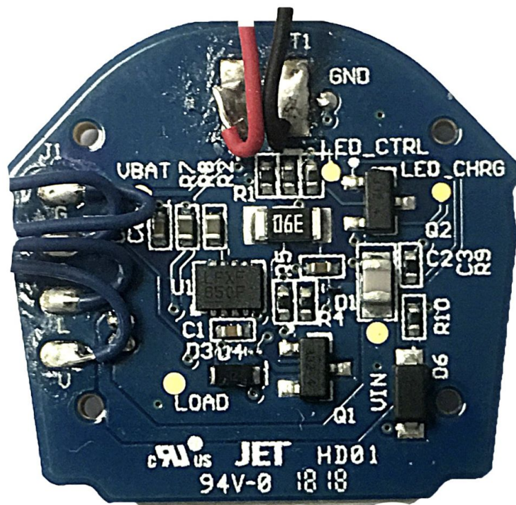
VPro+ RX Board (BOTTOM VIEW)
