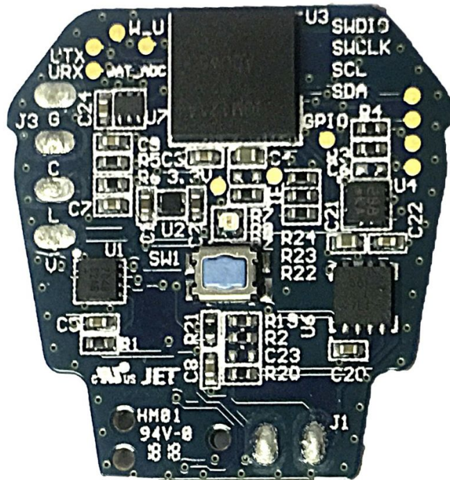
VPro+ Main Board: (TOP VIEW, SINGLE SIDE PCB)
