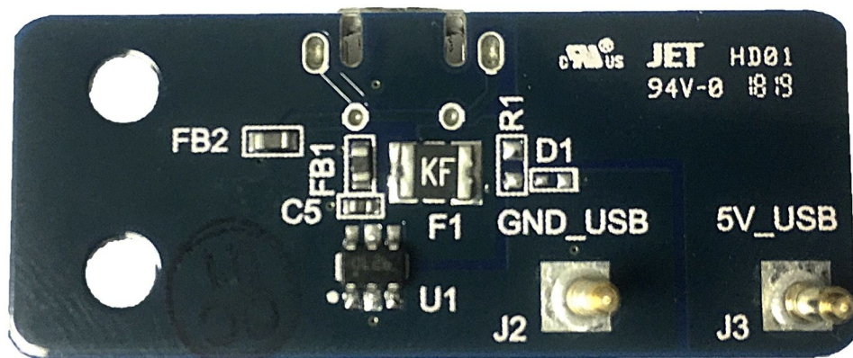
VPro+ USB Board: (BOTTOM SIDE)
