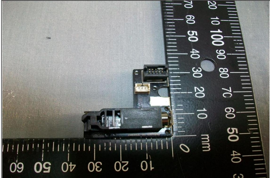
< Fan-F >
