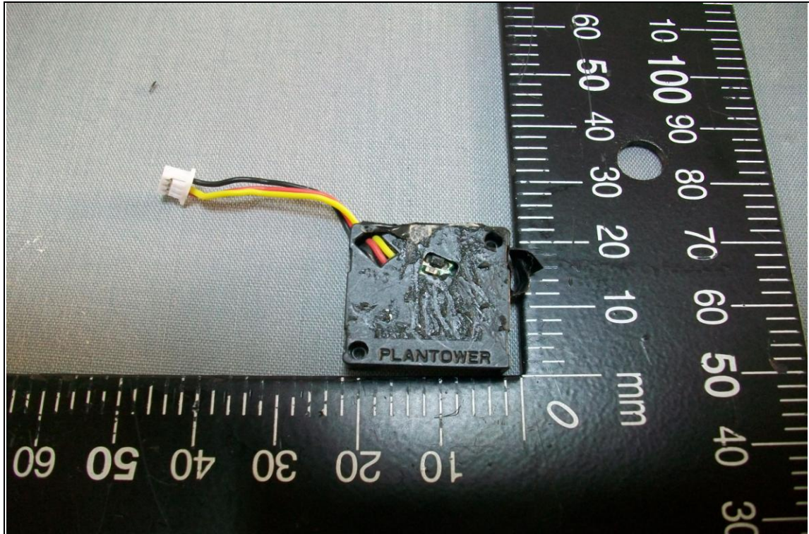
< Fan-R >
