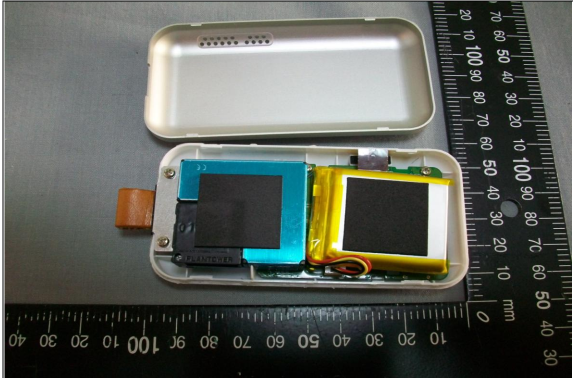
< Inside View >
