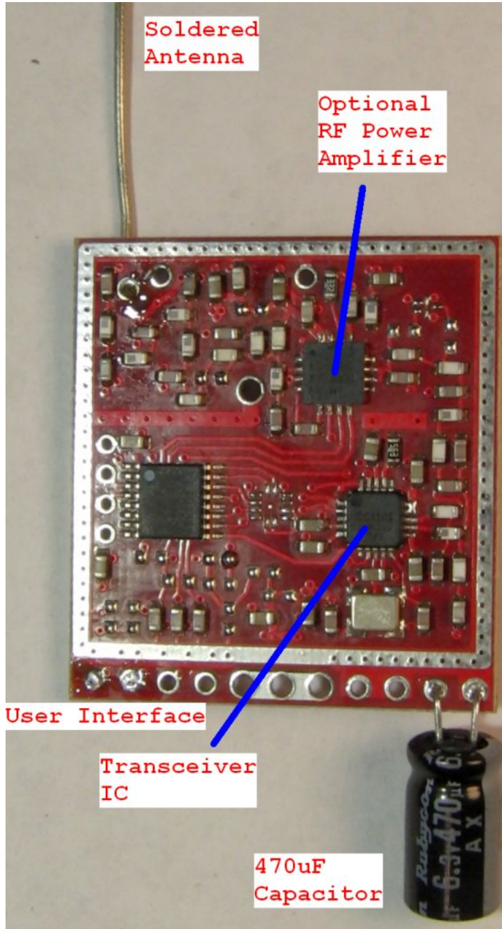
Figure E19.1 – Internal Photo – Module Top
