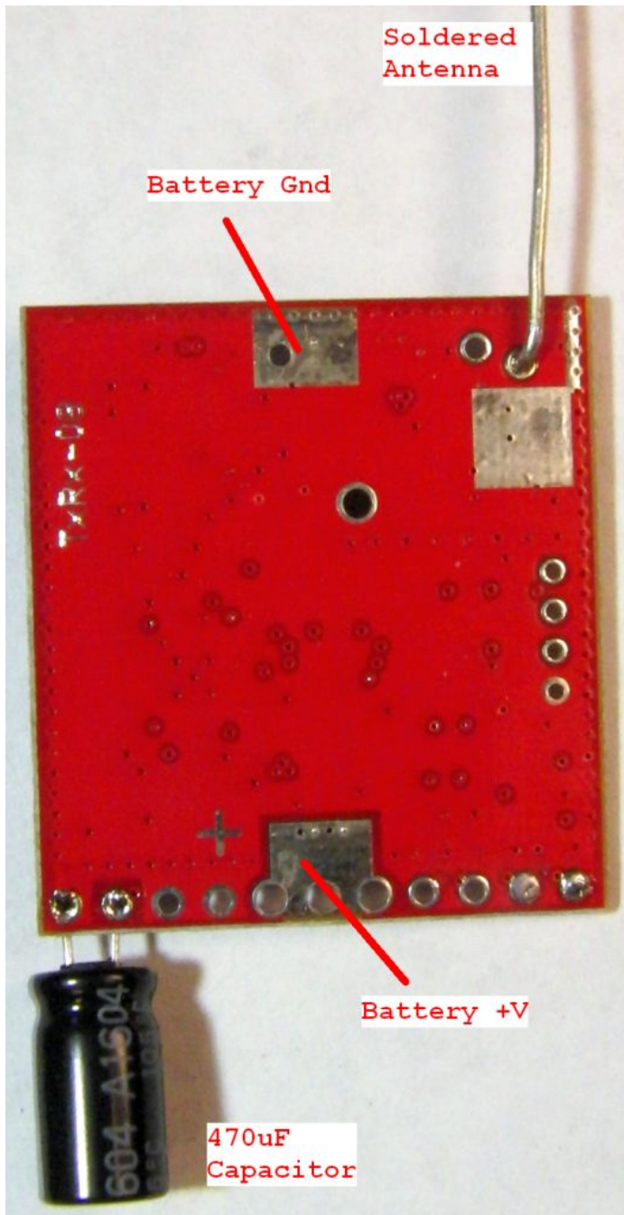
Figure E19.2 – Internal Photo – Module Bottom
