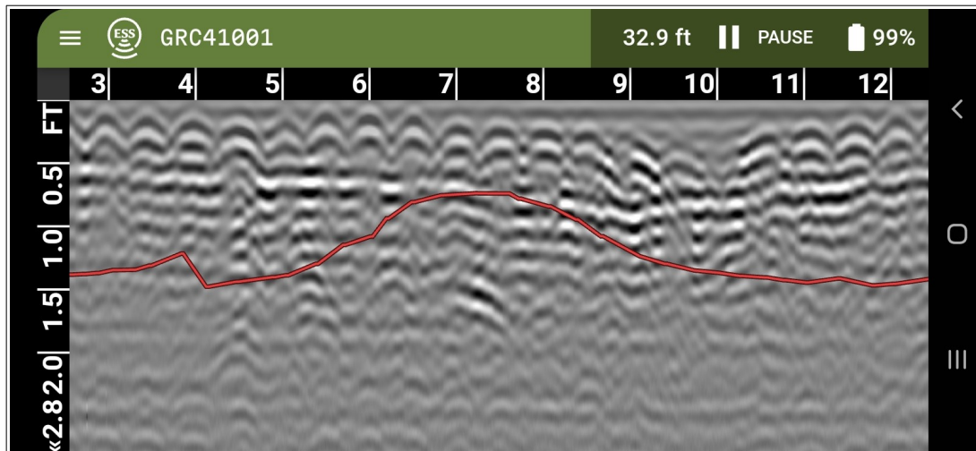
Figure 4: A GPR scan line on Surveyor Mobile . The red line plot indicates the detected magnetic signal of an electrical power line.
