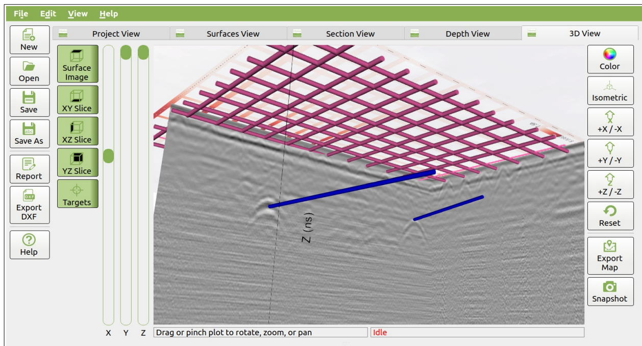
Figure 10: 3D data view from ESSential Underground.
