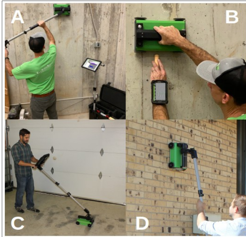
Figure 2: Different smart phone and tablet setups can be used for different survey types: A) Extension handle with tablet on floor stand, B) wrist-mounted smartphone, C) Extension-handle mounted tablet, D) Extension handle.
