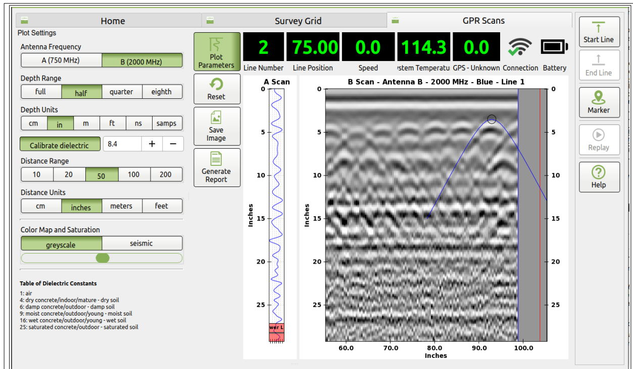
Figure 8: Plot settings dock. After clicking Calibrate dielectric , touch the top of a hyperbola. Then touch \pm or \pm until blue hyperbola matches the reflected radar arrivals on the screen.
