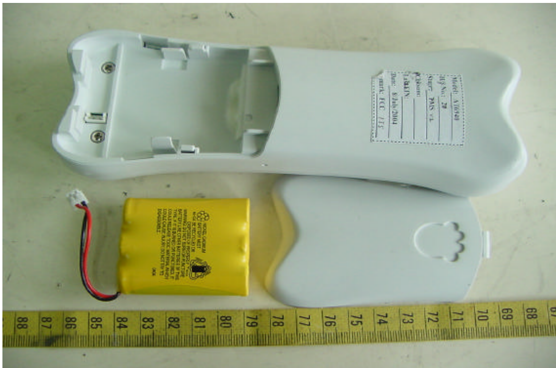
Internal View of Handset Unit
