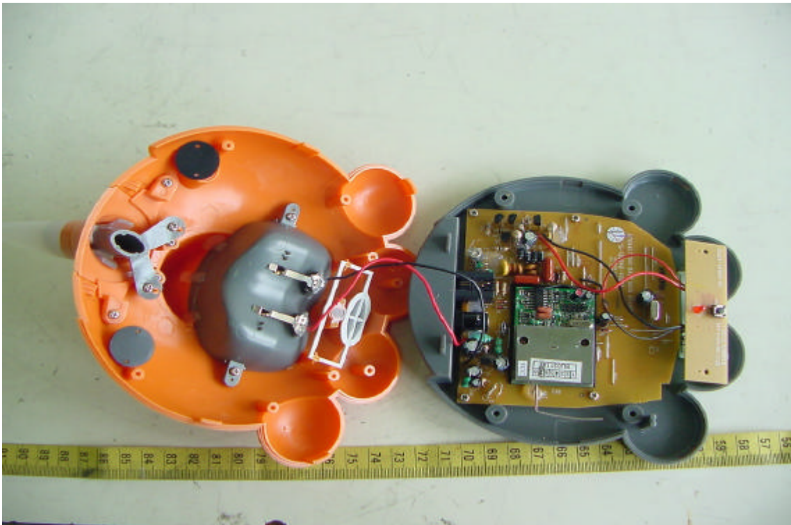
Internal View of Base Unit
