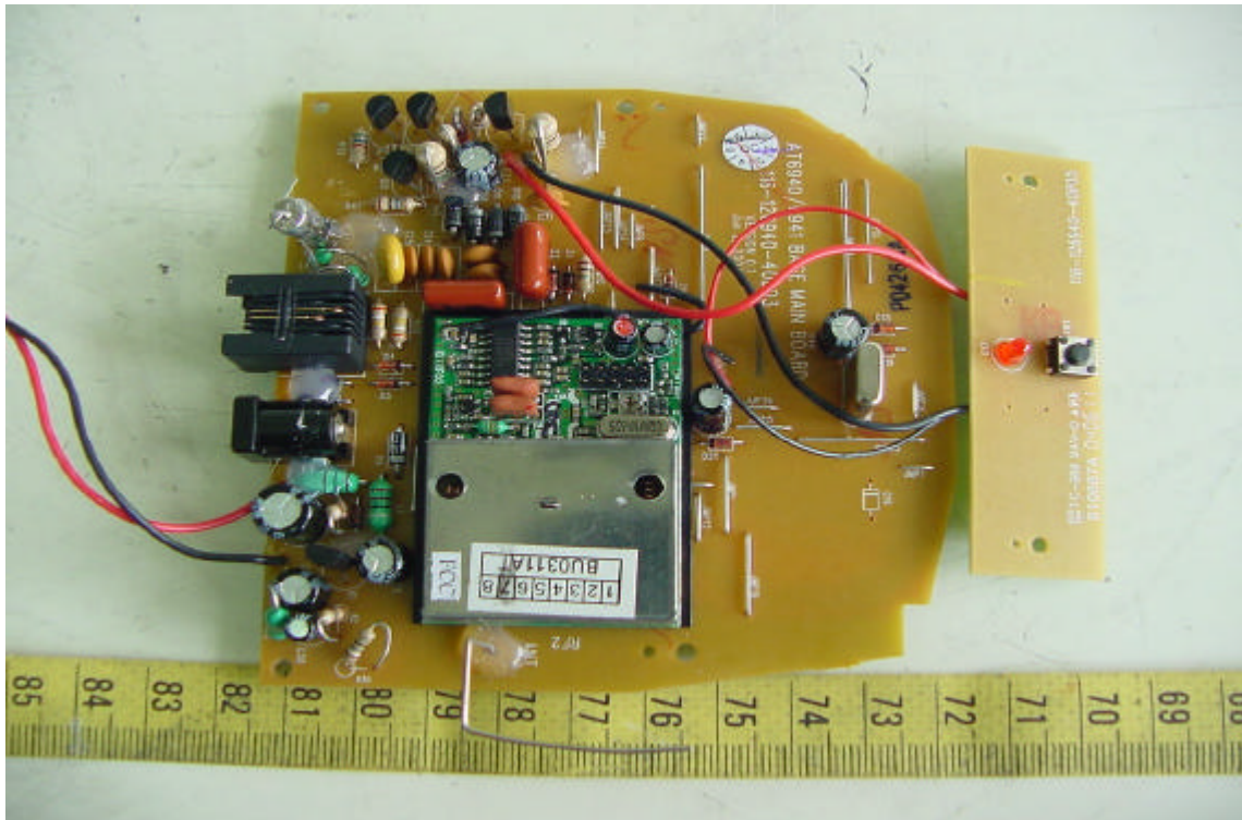
Component View of Base Unit's Main PCB
