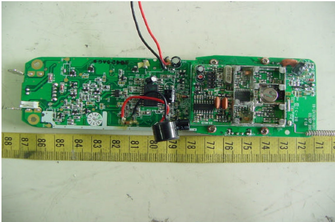
Solder View of Handset Unit's Main PCB
