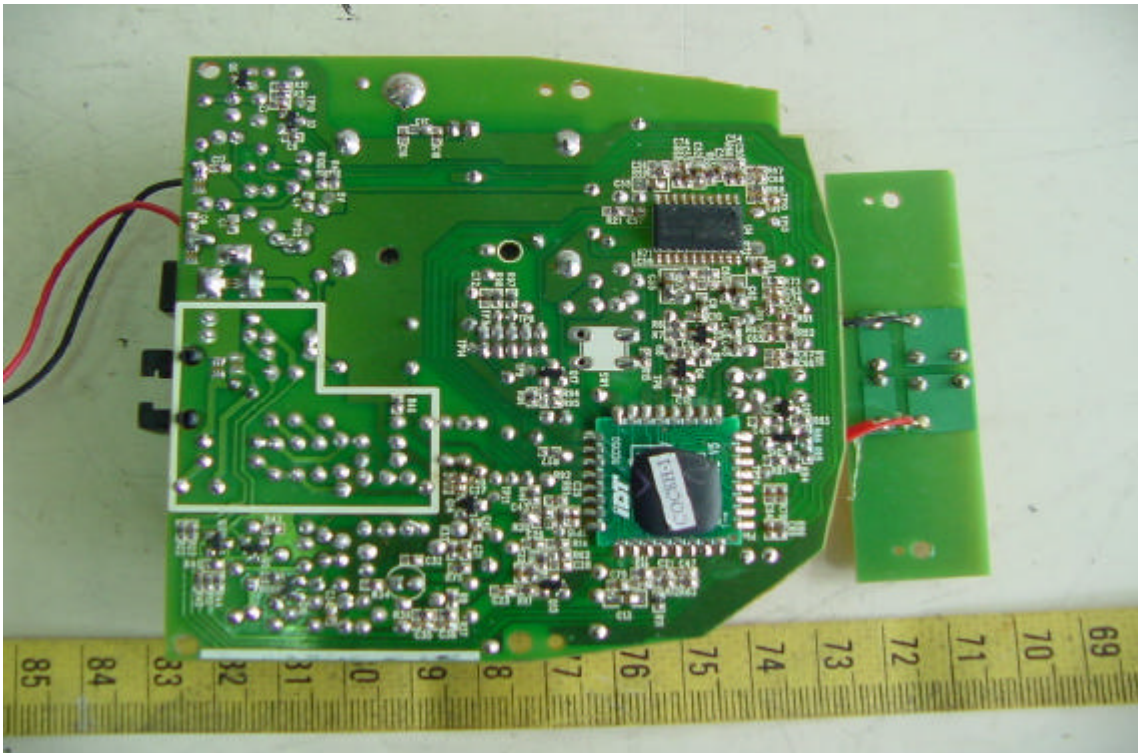
Solder View of Base Unit's Main PCB
