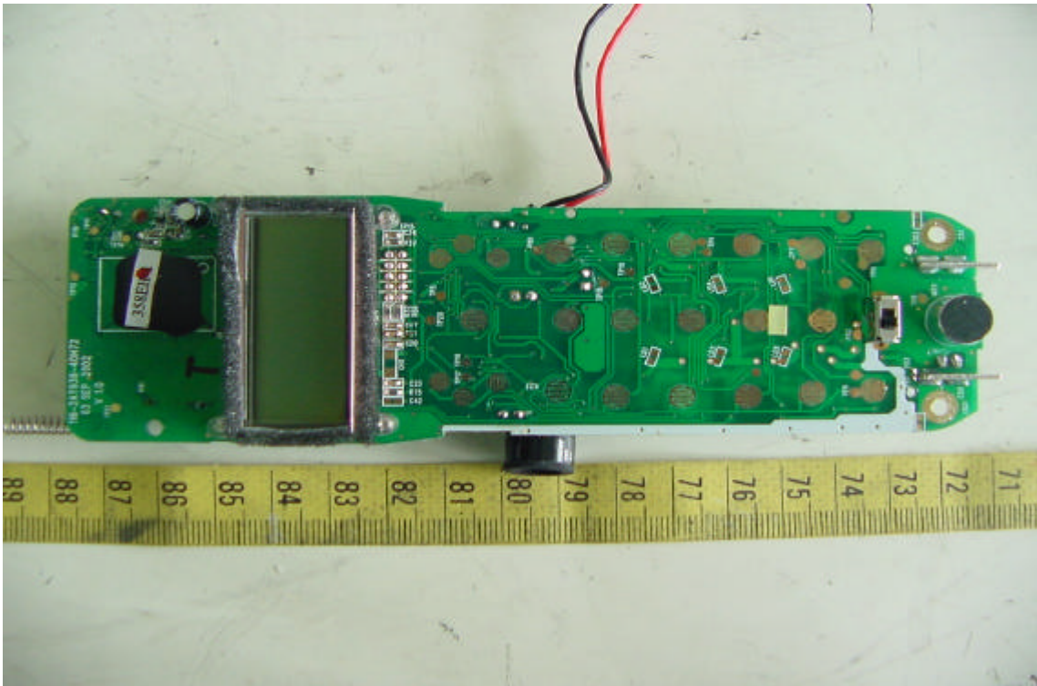
Component View of Handset Unit's Main PCB
