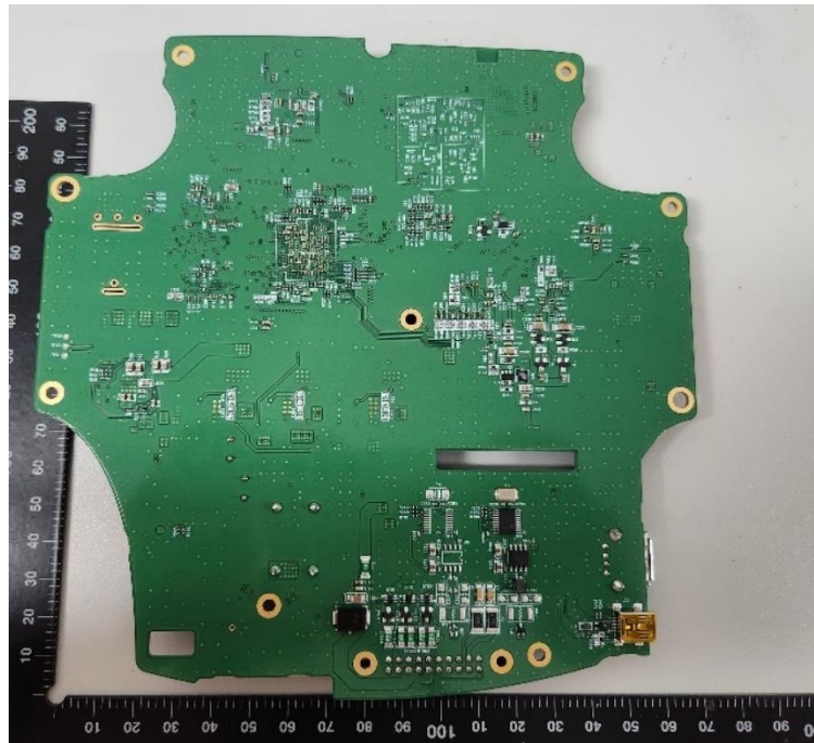
Main board - Rear Bottom
