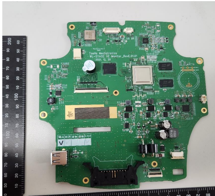
Main Board - Front Top
