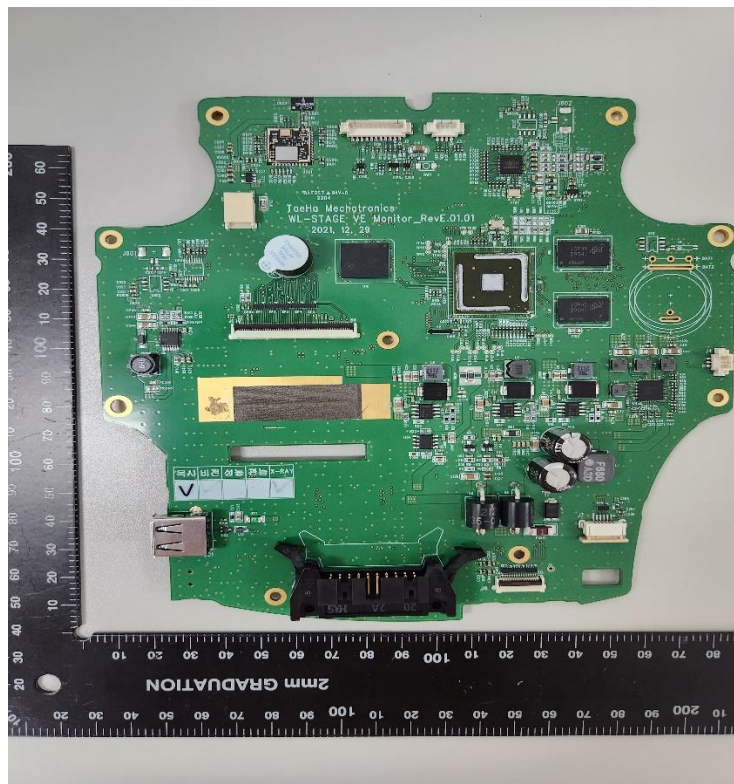
Main Board(Open Shield) - Front Top
