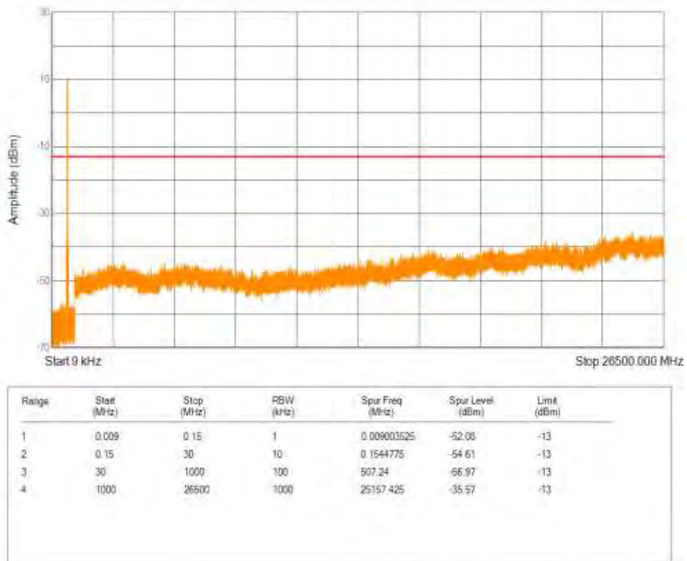
Band71 QPSK BW=20MHz Channel=133372 RB Size=100 Position=#0
