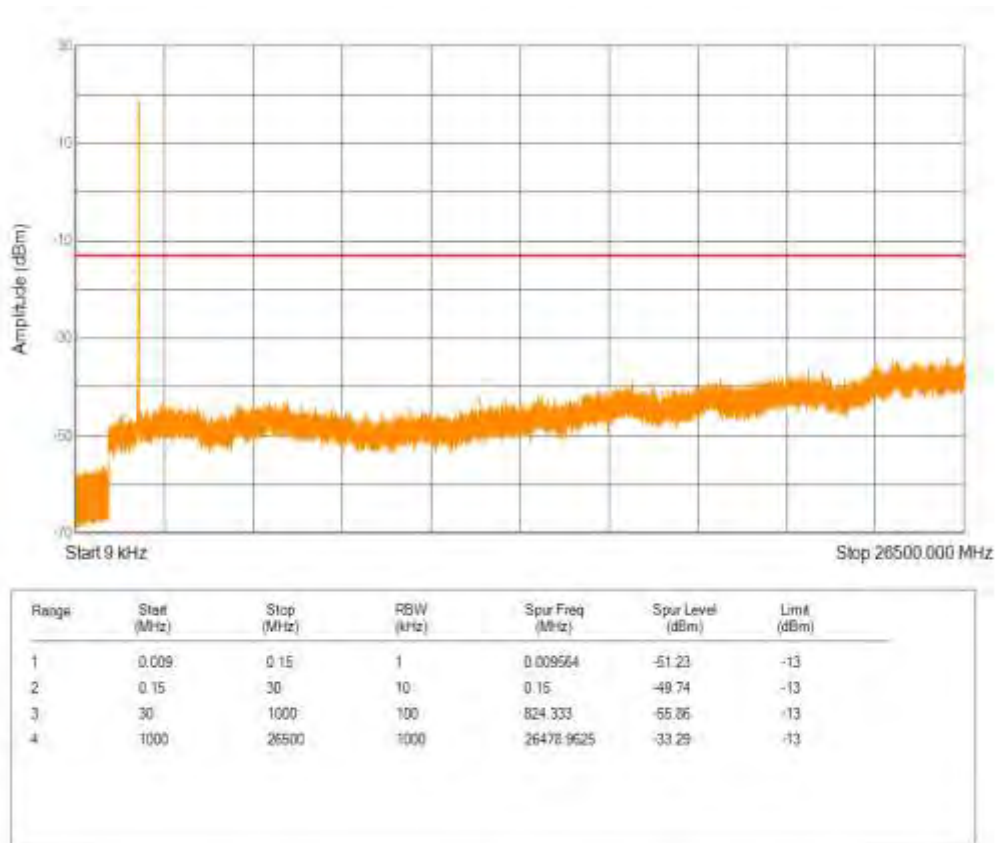
Band25 QPSK BW=20MHz Channel=26140 RB Size=100 Position=#0
