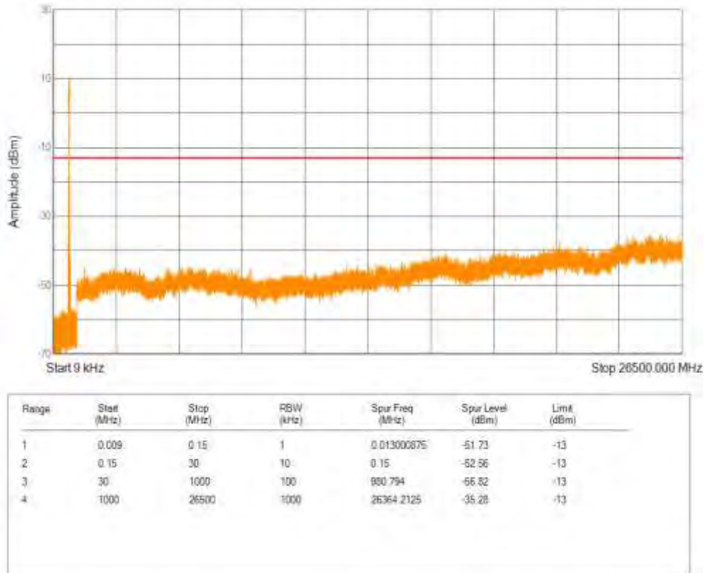
Band71 QPSK BW=20MHz Channel=133297 RB Size=100 Position=#0
