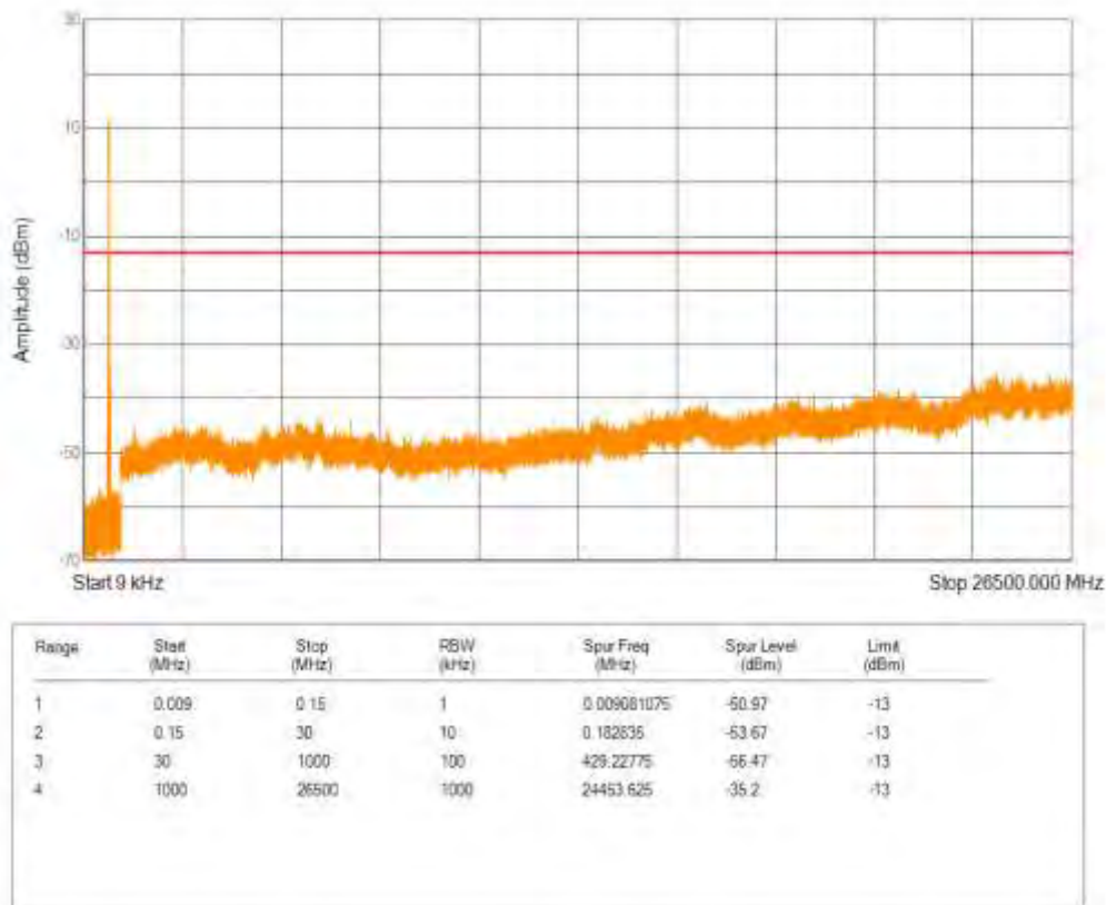
Band71 QPSK BW=20MHz Channel=133222 RB Size=100 Position=#0
