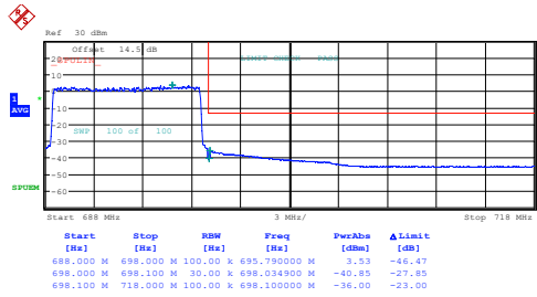
10MHz_High_QPSK_50@0
