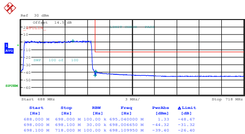
10MHz_High_16QAM_50@0
