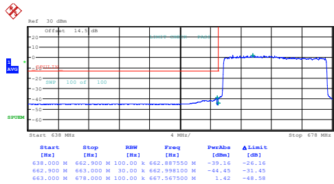
15MHz_Low_QPSK_75@0
