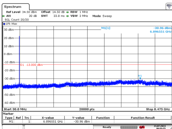
2_3MHz_High_QPSK_15@0
