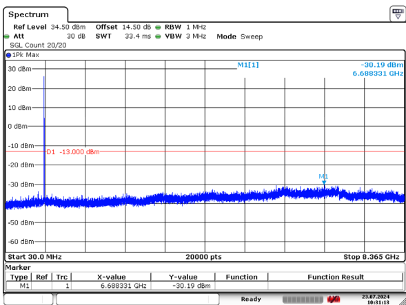
2_3MHz_Middle_QPSK_1@0
