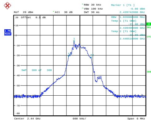
Middle 1.026MHz
