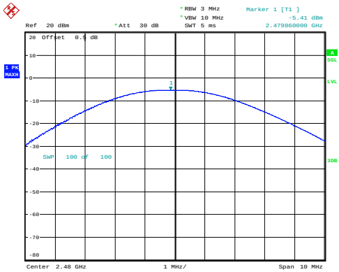
High -5.41dBm
