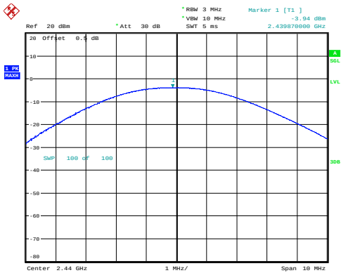
Middle -3.94dBm
