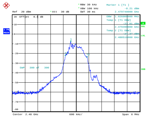
High 1.026MHz
