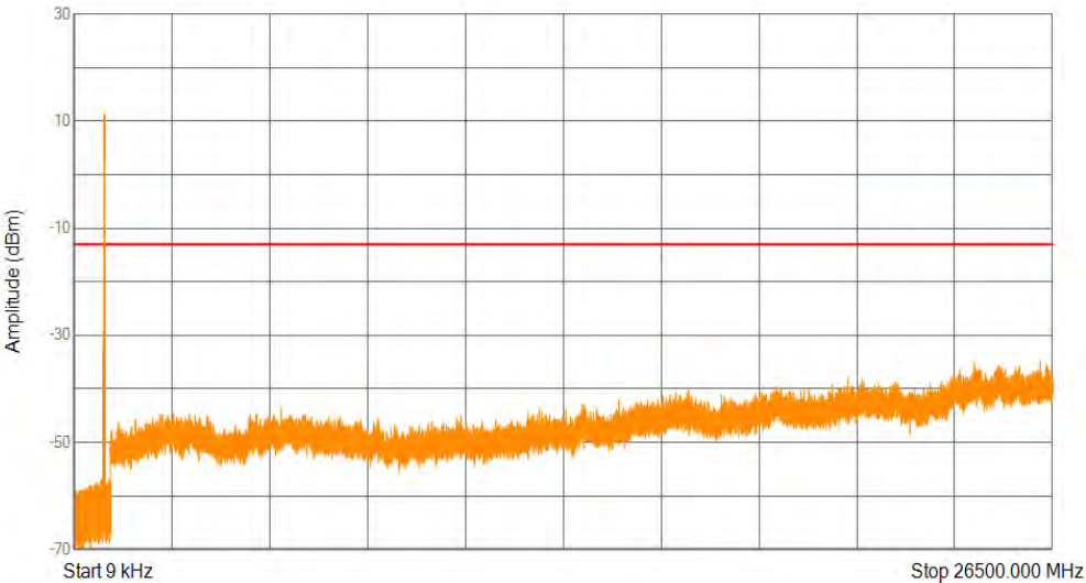
Band26(824-849) QPSK BW=15MHz Channel=26915 RB Size=75 Position=#0
