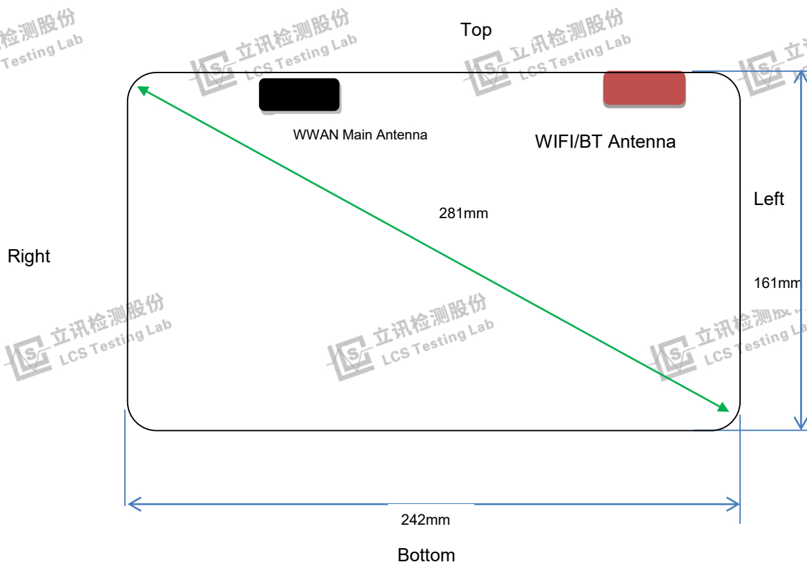
Rear View
