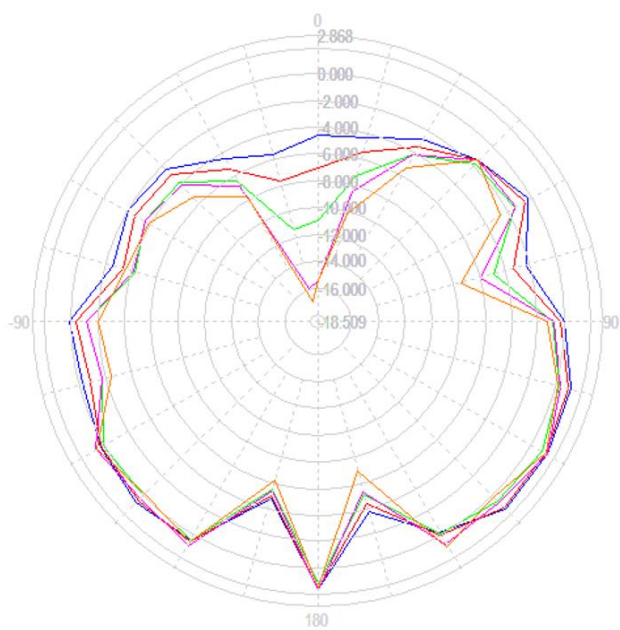
- E1 Plane Polar/Line Chart -
