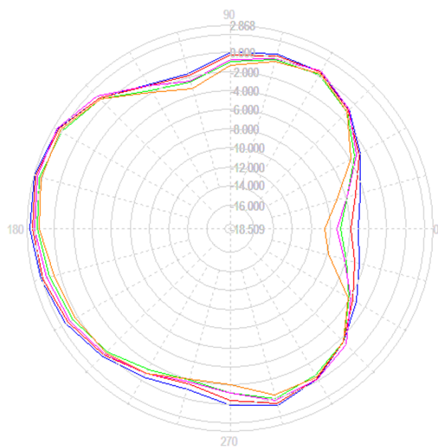
- H Plane Polar/Line Chart -
