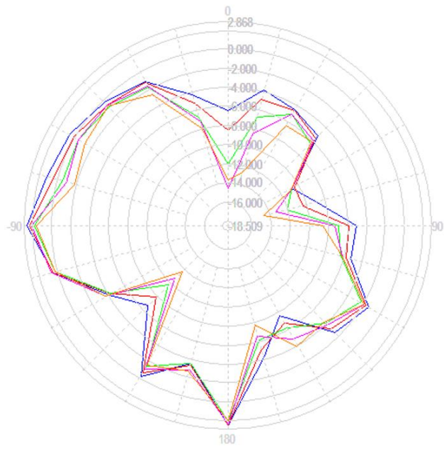
- E2 Plane Polar/Line Chart -
