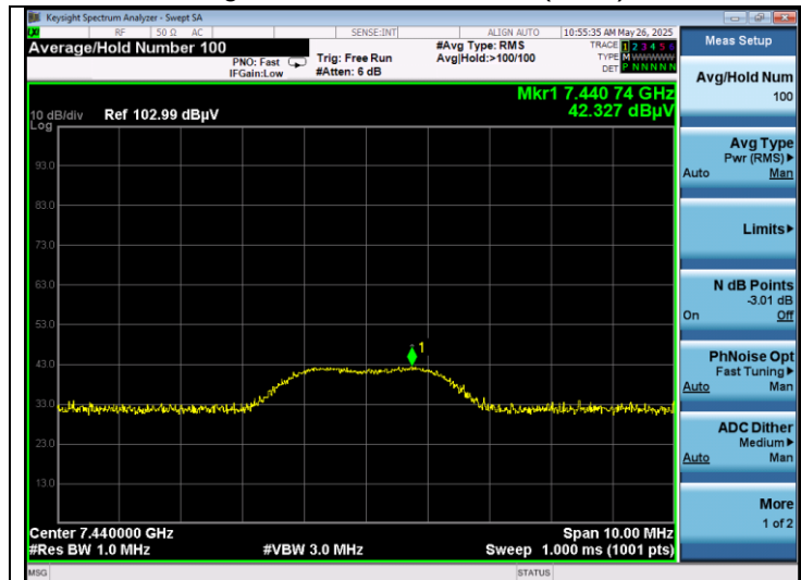
High channel 3 rd harmonic (Peak)
