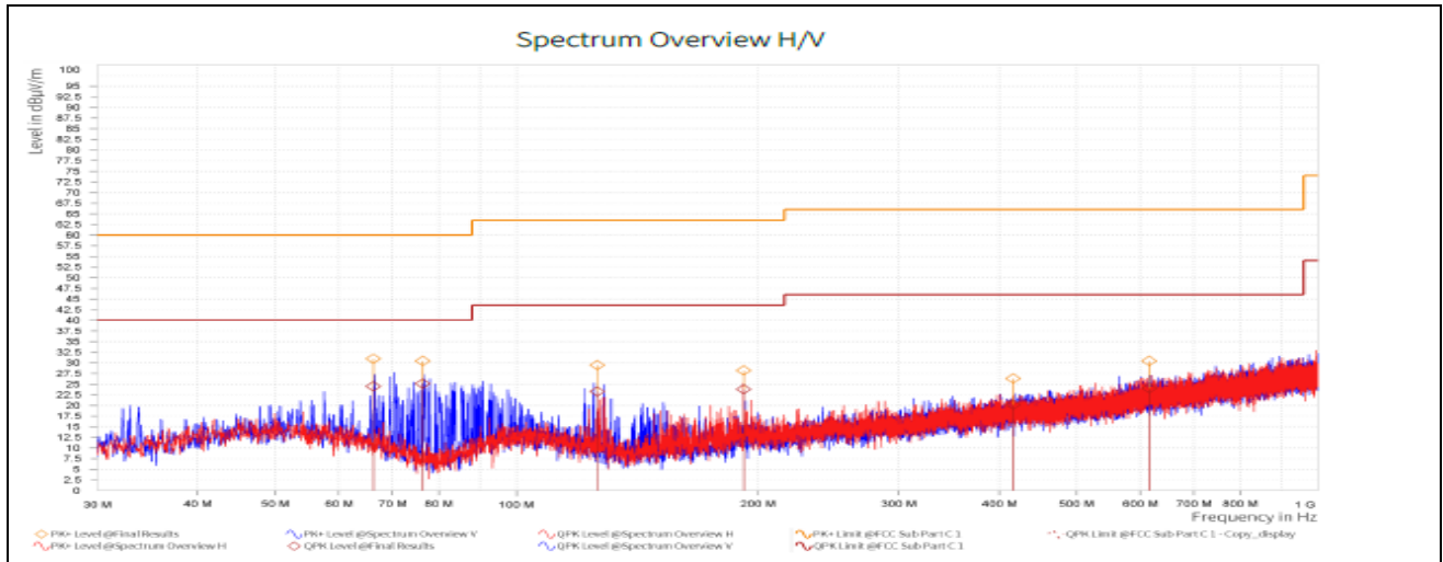
30 MHz – 1 GHz
