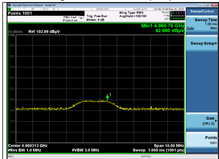
High channel 2 nd harmonic (Peak)
