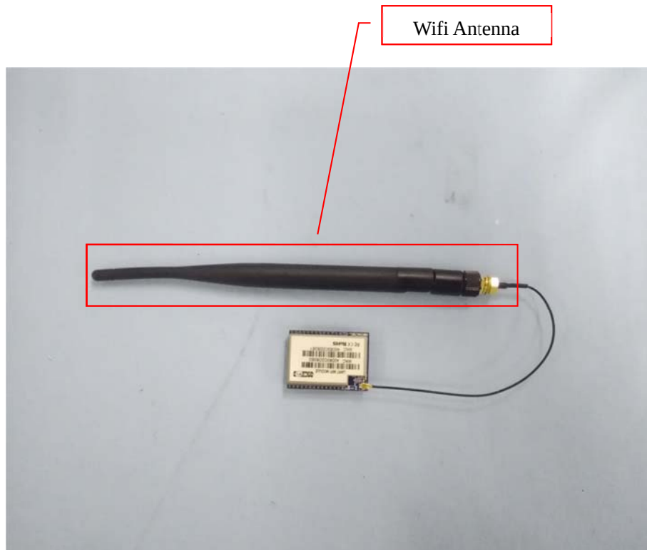
EUT View 1
