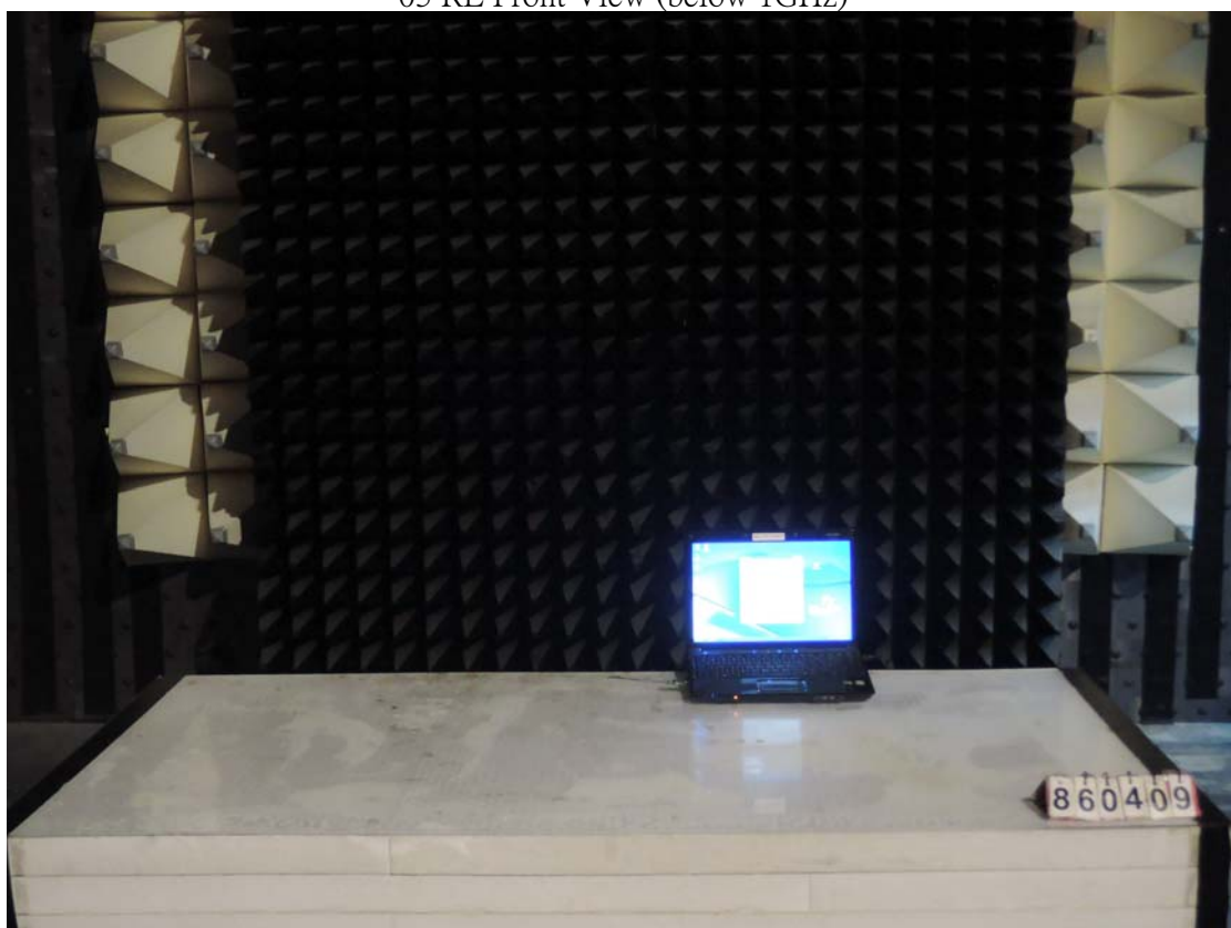
03 RE Front View (below 1GHz)
