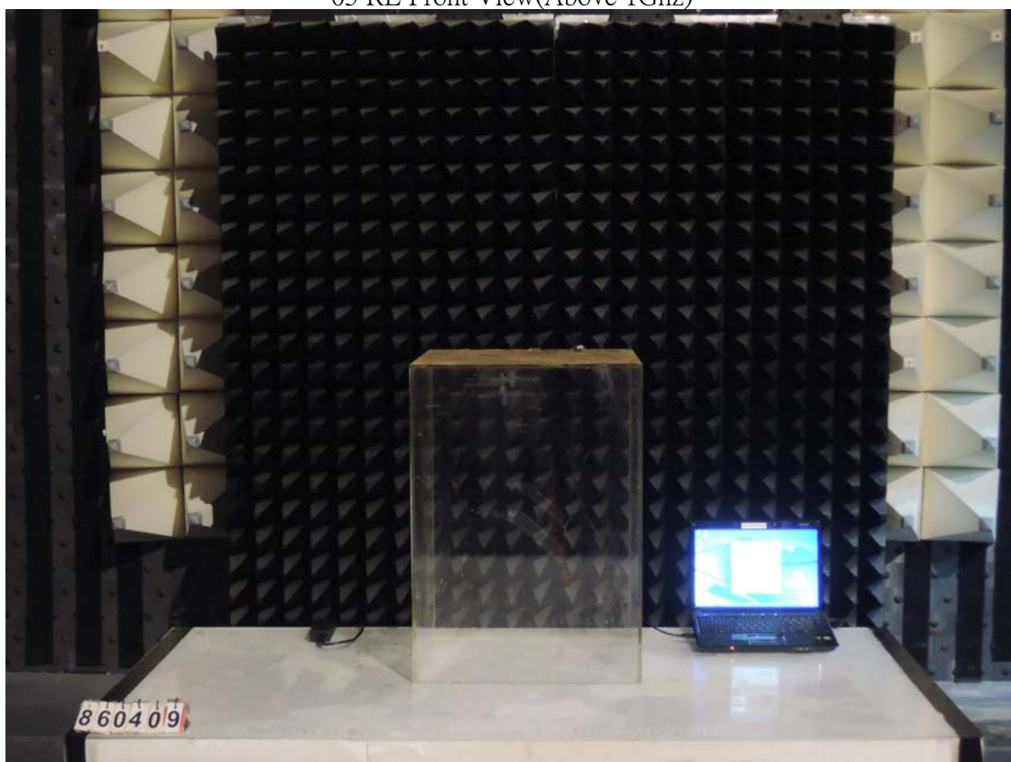
05 RE Front View(Above 1Ghz)
