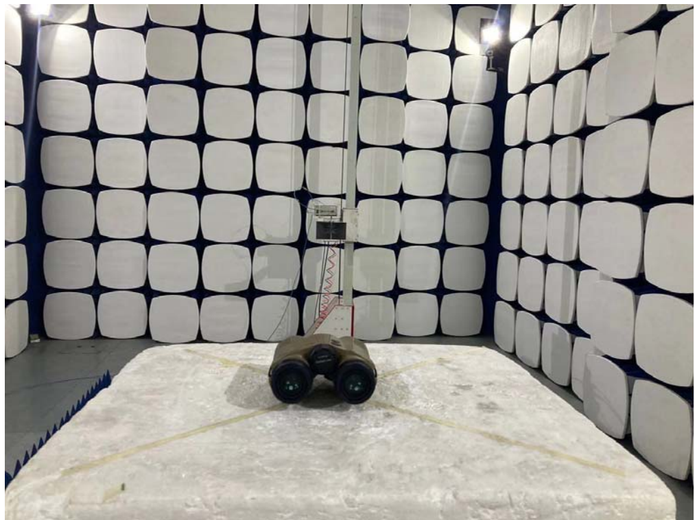
Radiated Setup photo (Above 1G)
