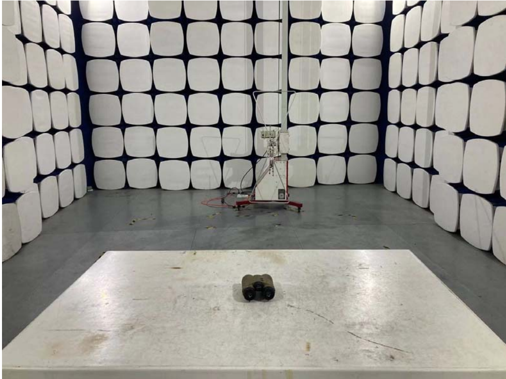
Radiated Setup photo (Below 1G)
