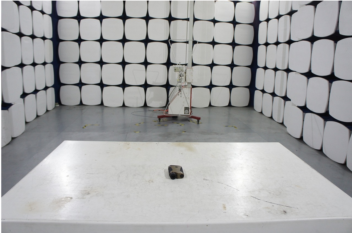
Radiated Setup photo (Below 1G)
