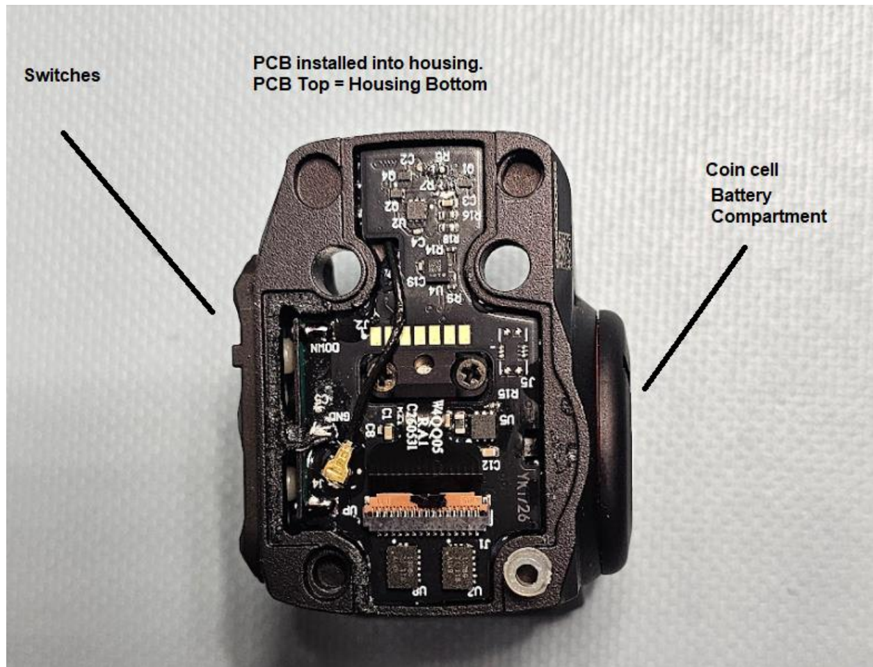
Board photos
