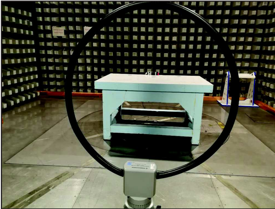
Photo 2: Antenna 90° to EUT
