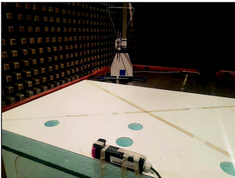
Photo 4: Antenna V Polarization to EUT
