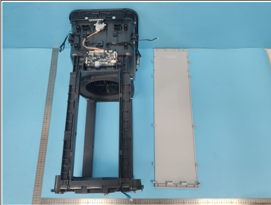
Fig. 33 Disassembly view
