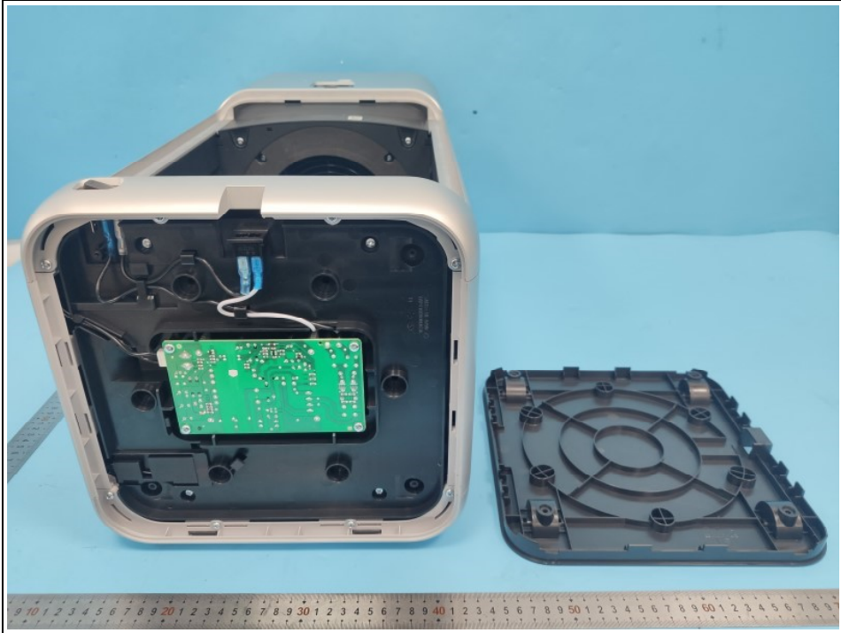
Fig.12 Disassembly view
