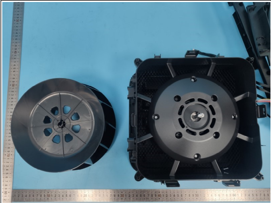
Fig. 45 Disassembly view
