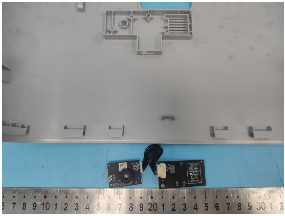
Fig. 26 Disassembly view
