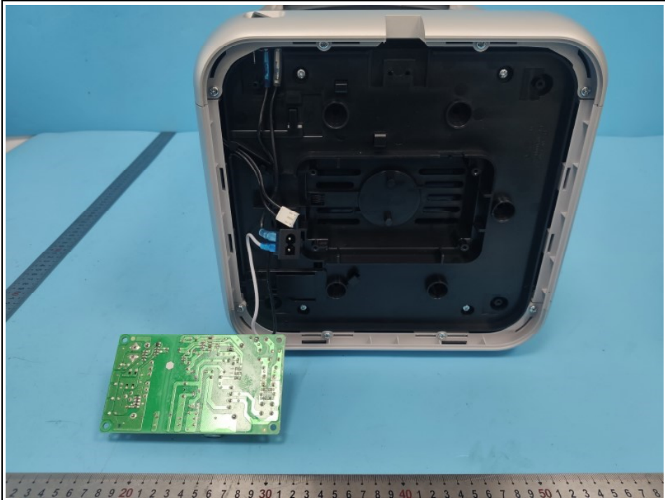
Fig.15 Disassembly view
