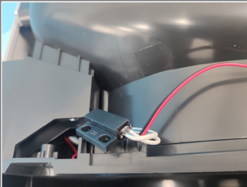
Fig. 28 Disassembly view
