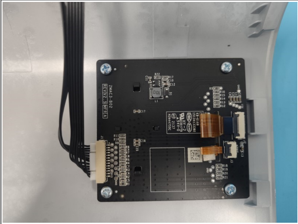
Fig. 30 Display board
