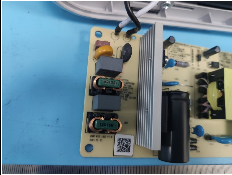
Fig.18 Switching power supply board
