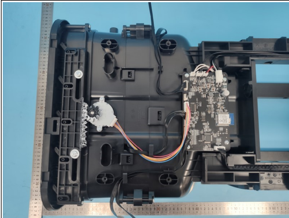
Fig. 37 Disassembly view
