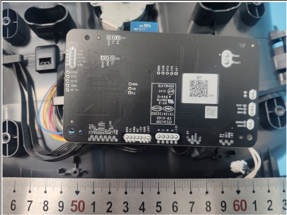
Fig. 39 Main control board
