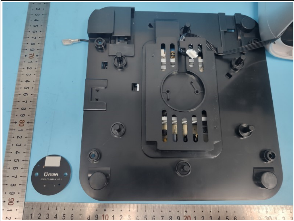
Fig.23 Disassembly view
