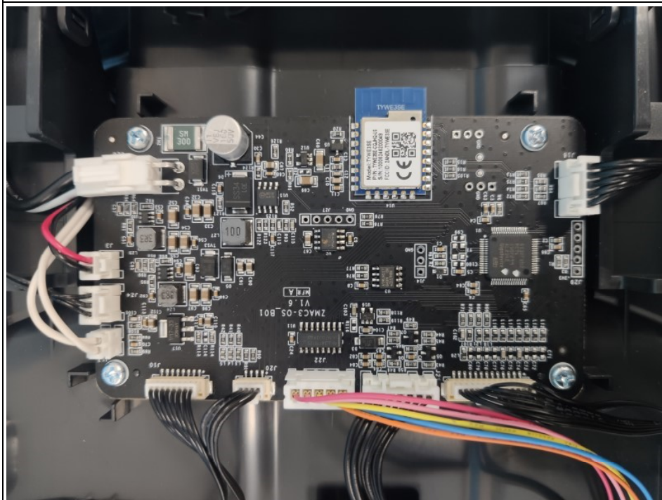
Fig. 38 Main control board
