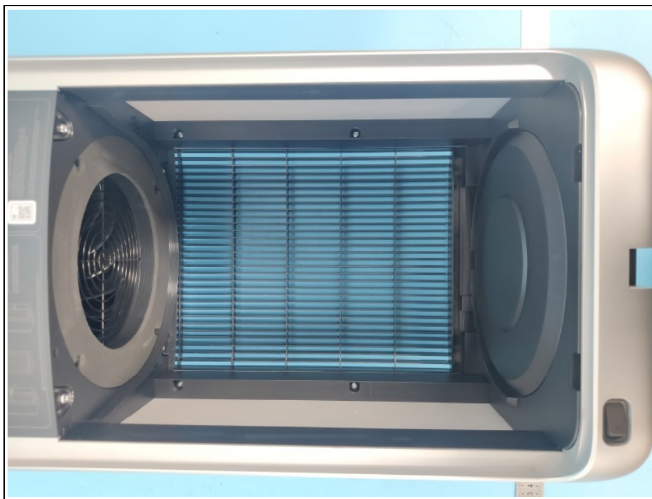
Fig.9 Disassembly view
