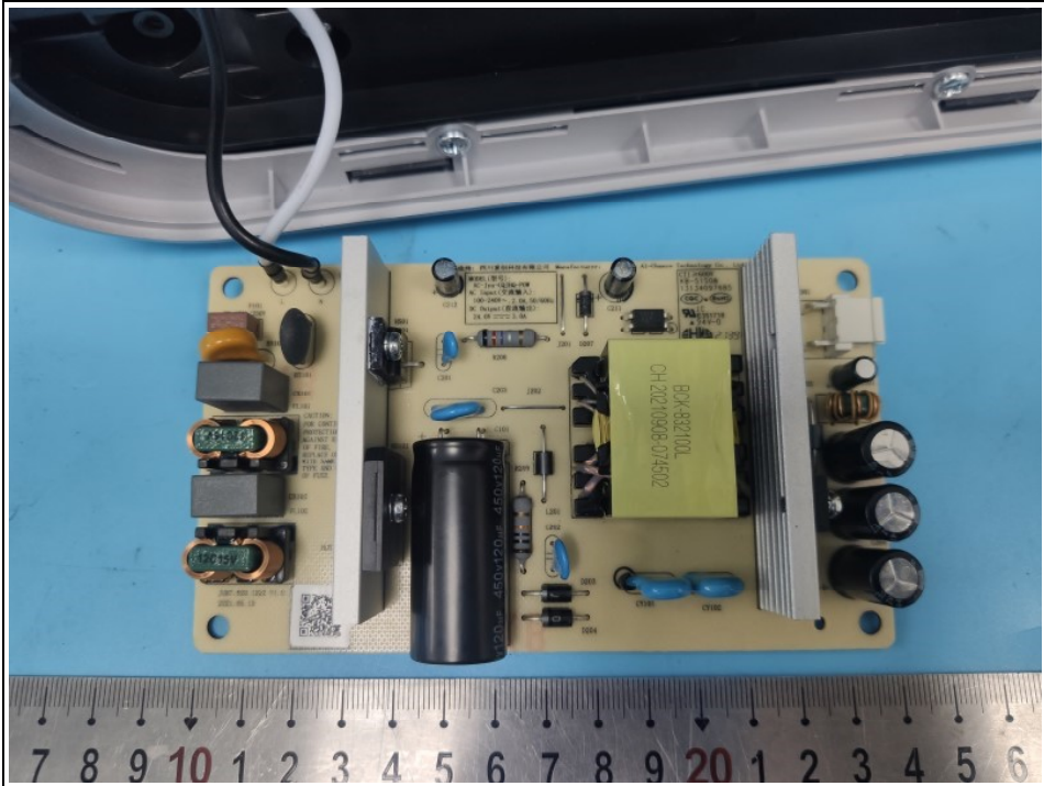
Fig.17 Switching power supply board
