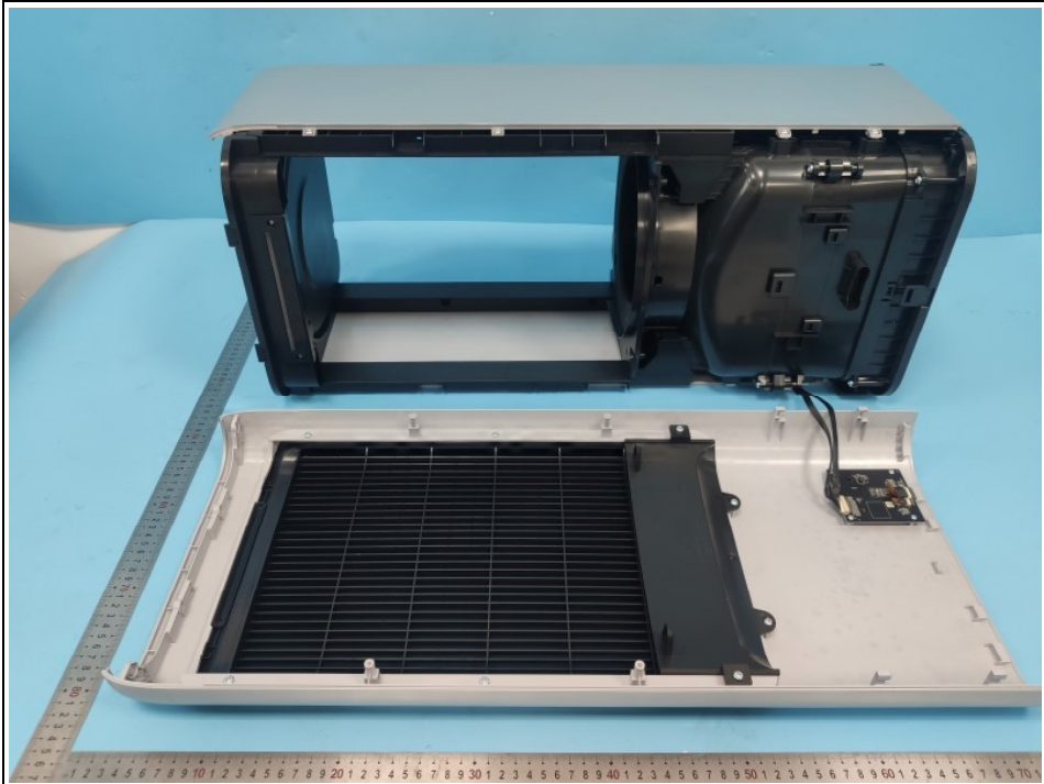
Fig. 29 Disassembly view
