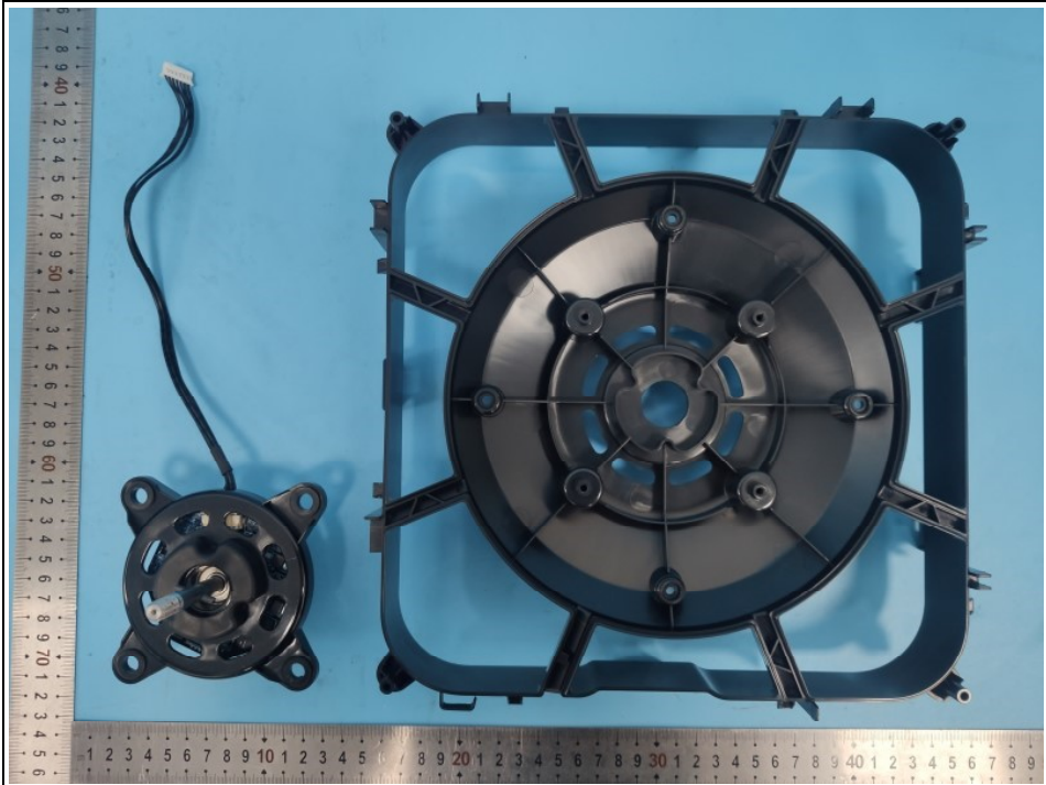
Fig. 47 Disassembly view
