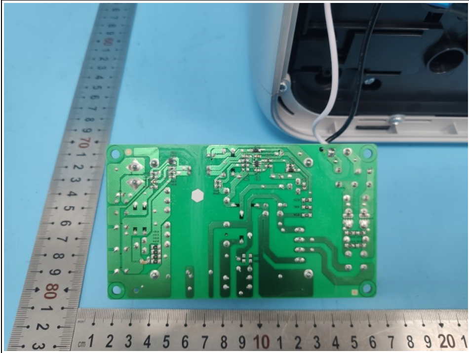
Fig.16 Switching power supply board
