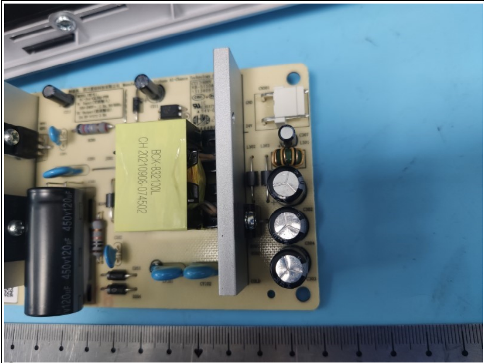
Fig.19 Switching power supply board
