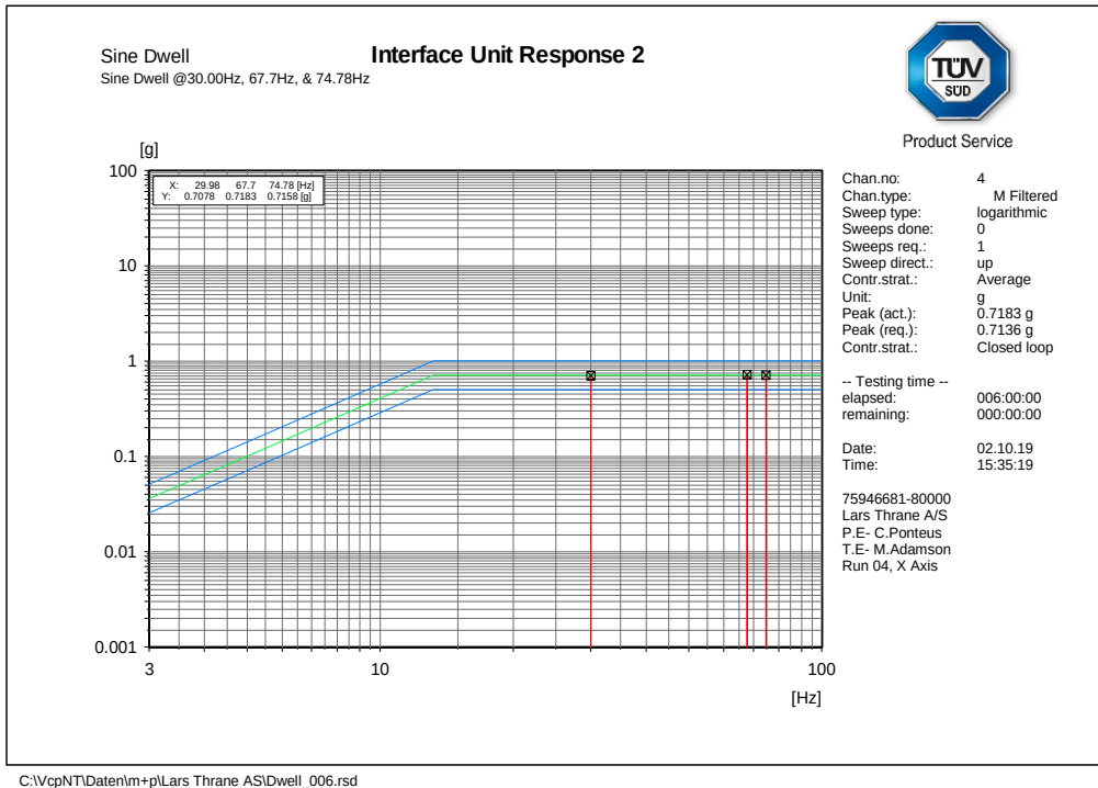
Figure 2.8.6 Run 04, X axis, Dwell
