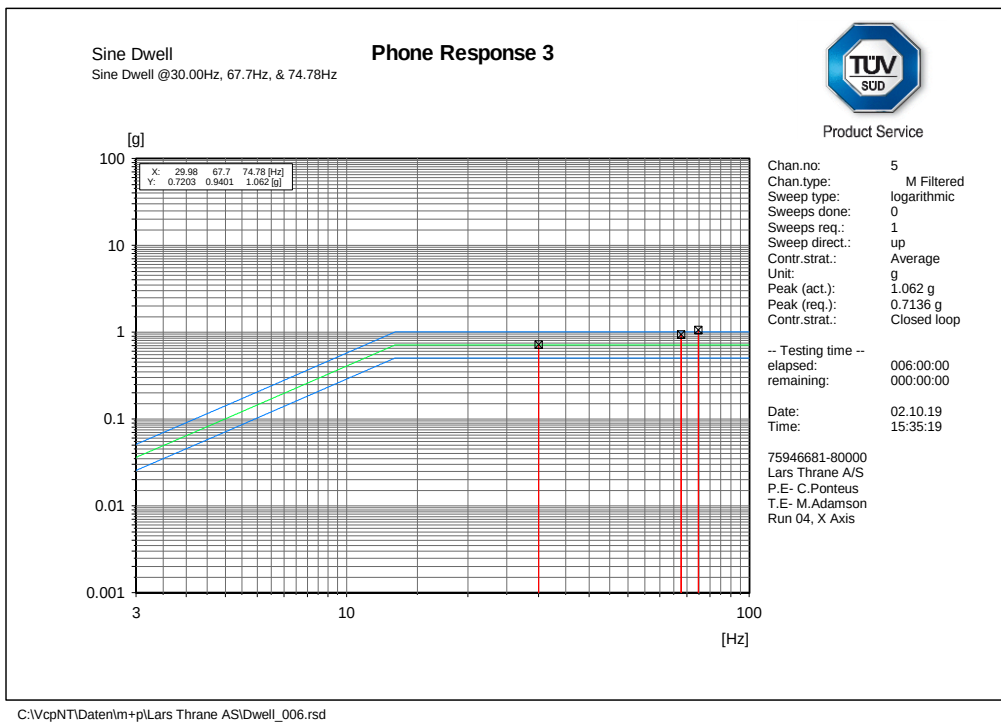
Figure 2.8.7 Run 04, X axis, Dwell
