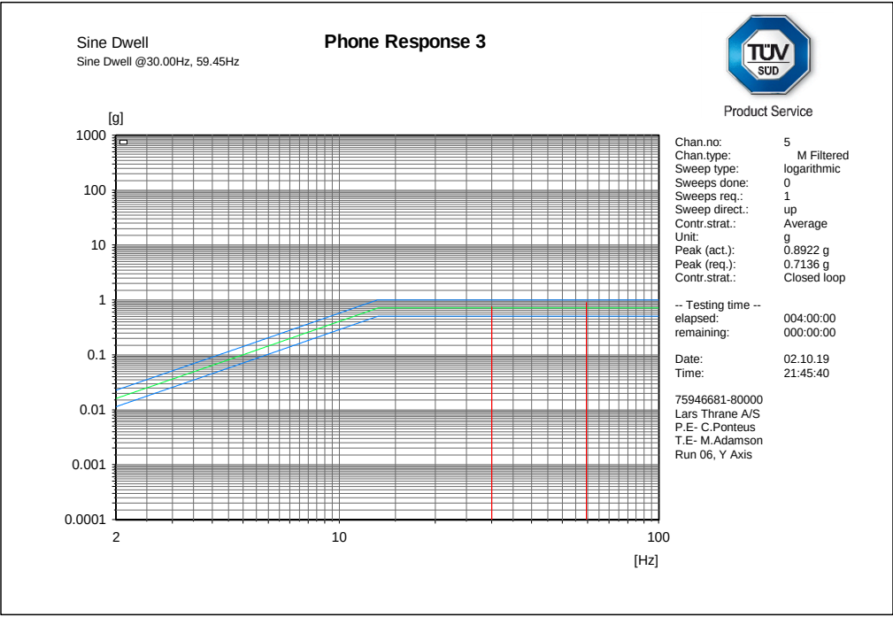
Figure 2.8.14 Run 06, Y axis, Dwell
