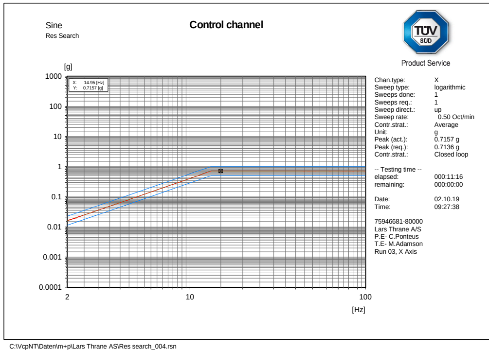
Figure 2.8.4 Run 03, X axis, Resonance sweep
