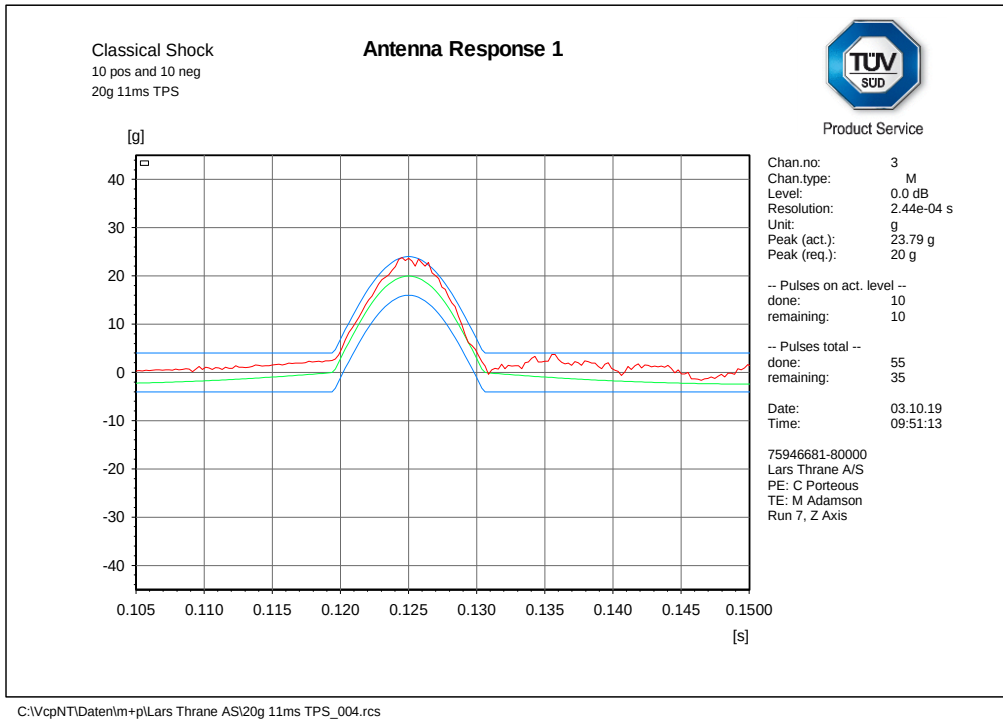
Figure 2.9.3 Run 07, Z axis, Shock +ve
