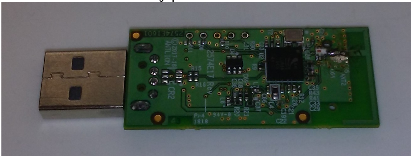
Photograph of PC Board: Foil Side
