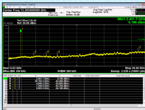
Lowest 30MH-26.5GHz
