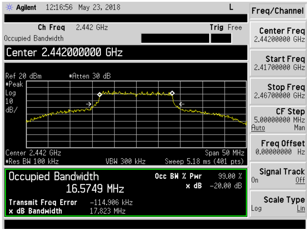
Figure 57. 20 dB Bandwidth – G mode Mid Channel
