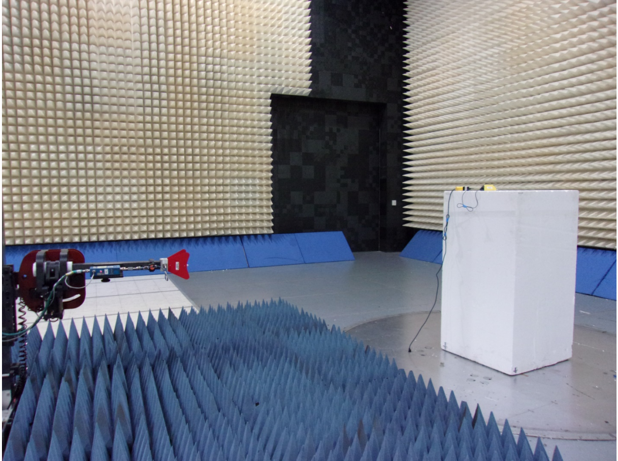
Intentional / spurious emissions, 1-18GHz
