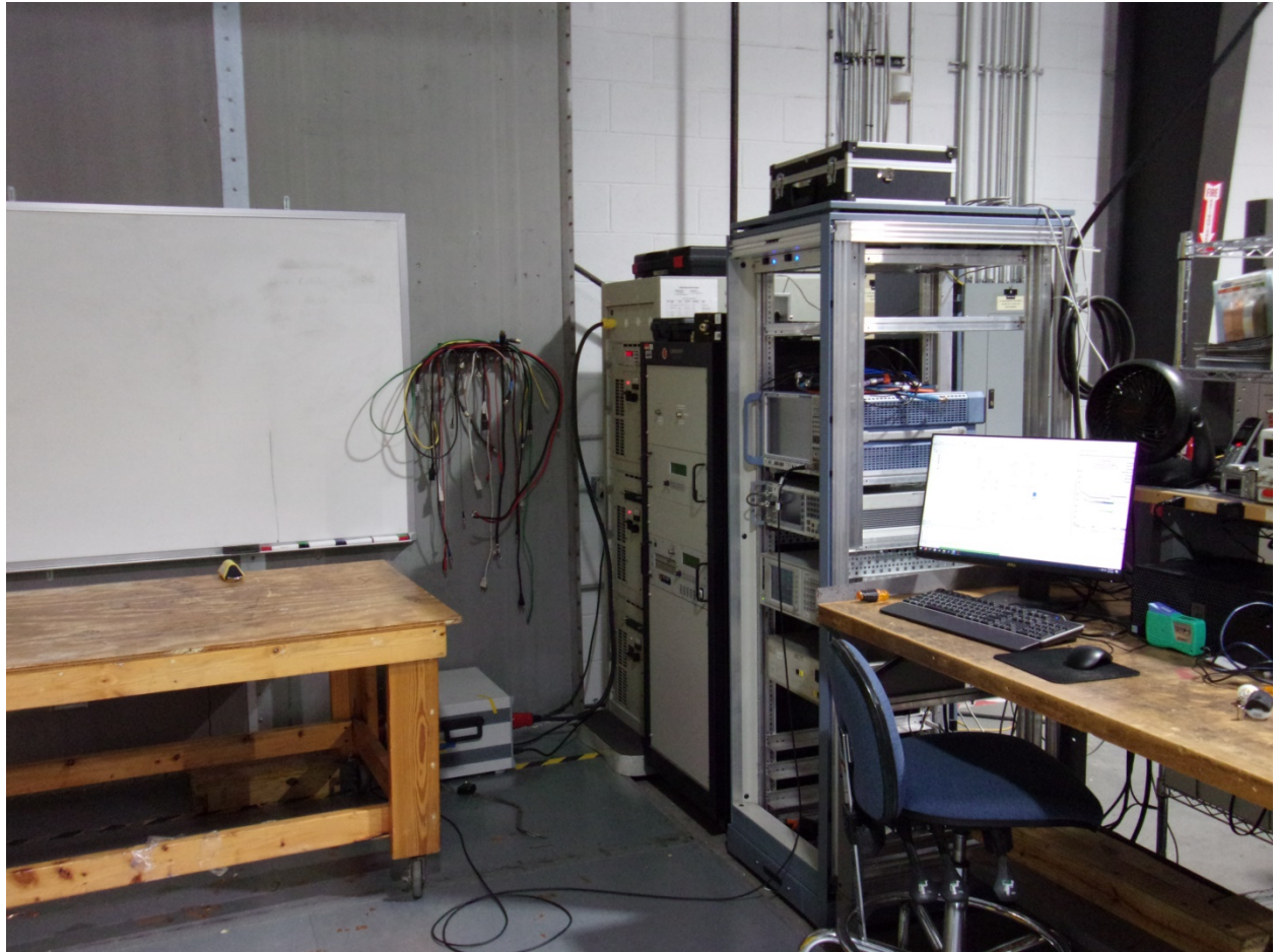
Conducted emissions, 150kHz-30MHz
