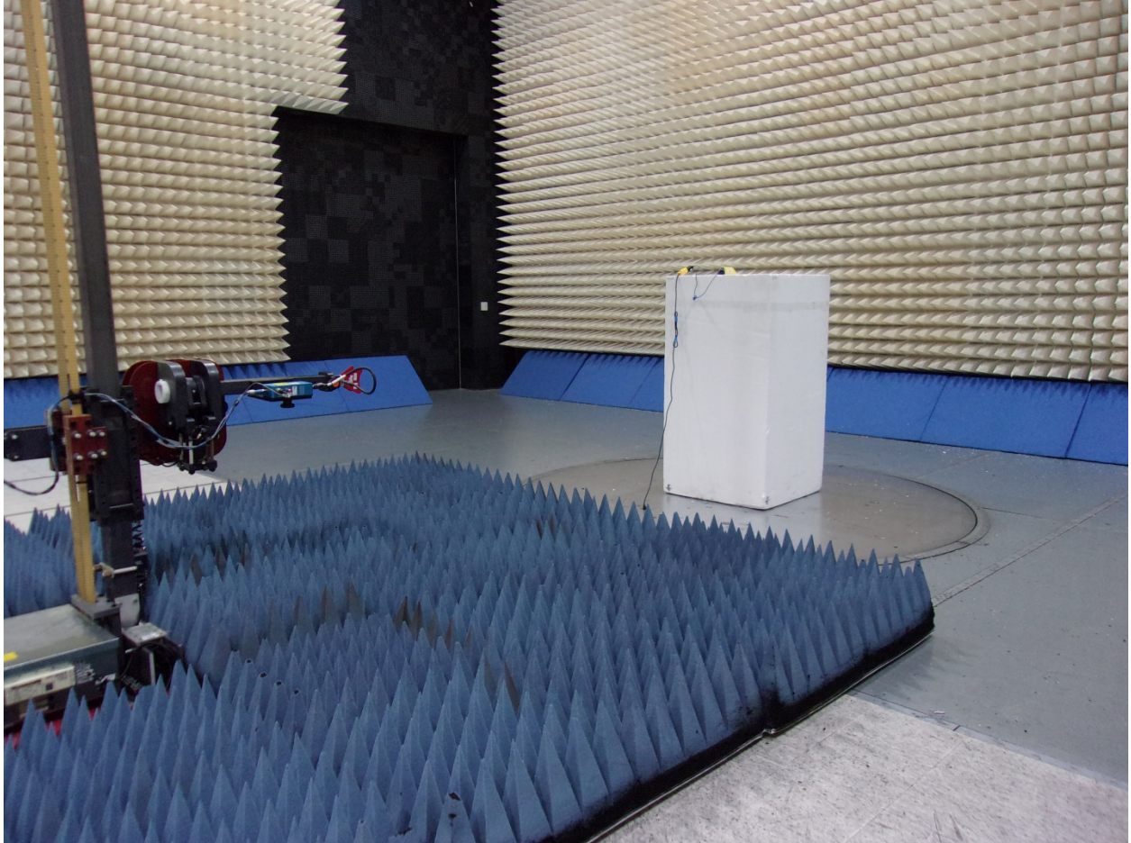
Intentional / spurious emissions, 18-29GHz
