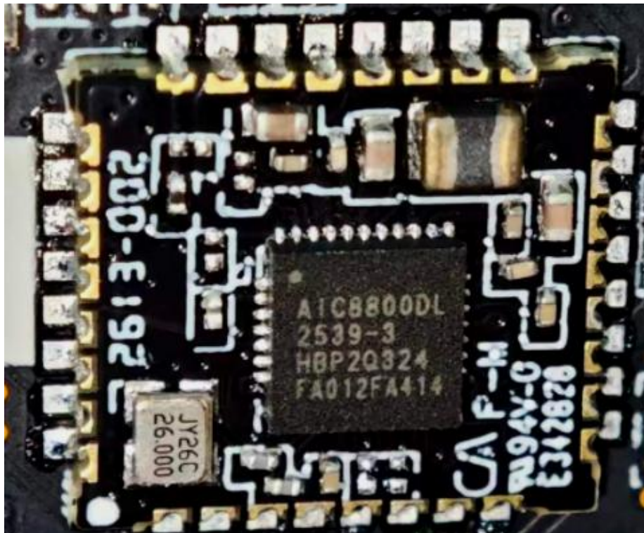
Internal Photos(Model No.:A531D)
