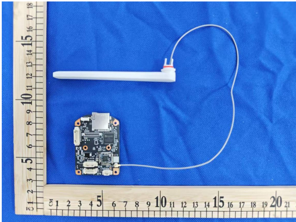
Internal Photos(Model No.:A531)
