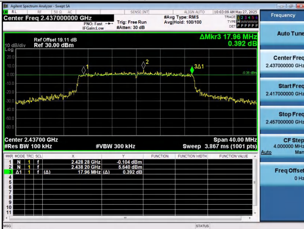
11AX20SISO-Ant1-2437-PASS
