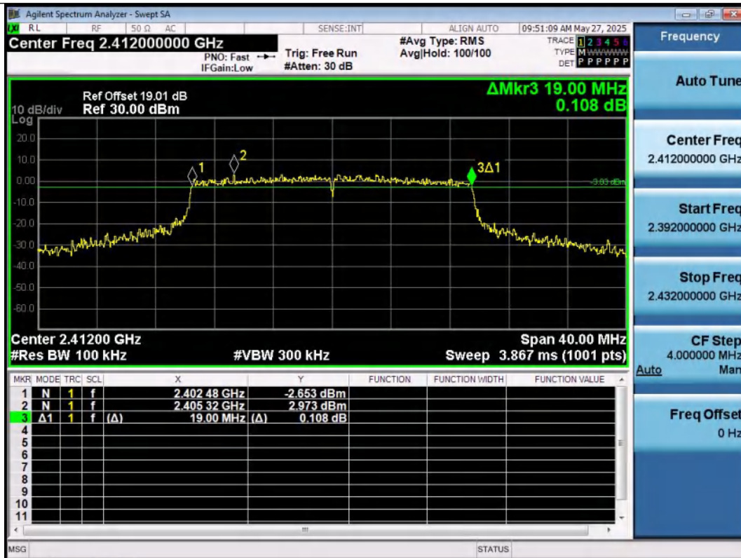
11AX20SISO-Ant1-2412-PASS
