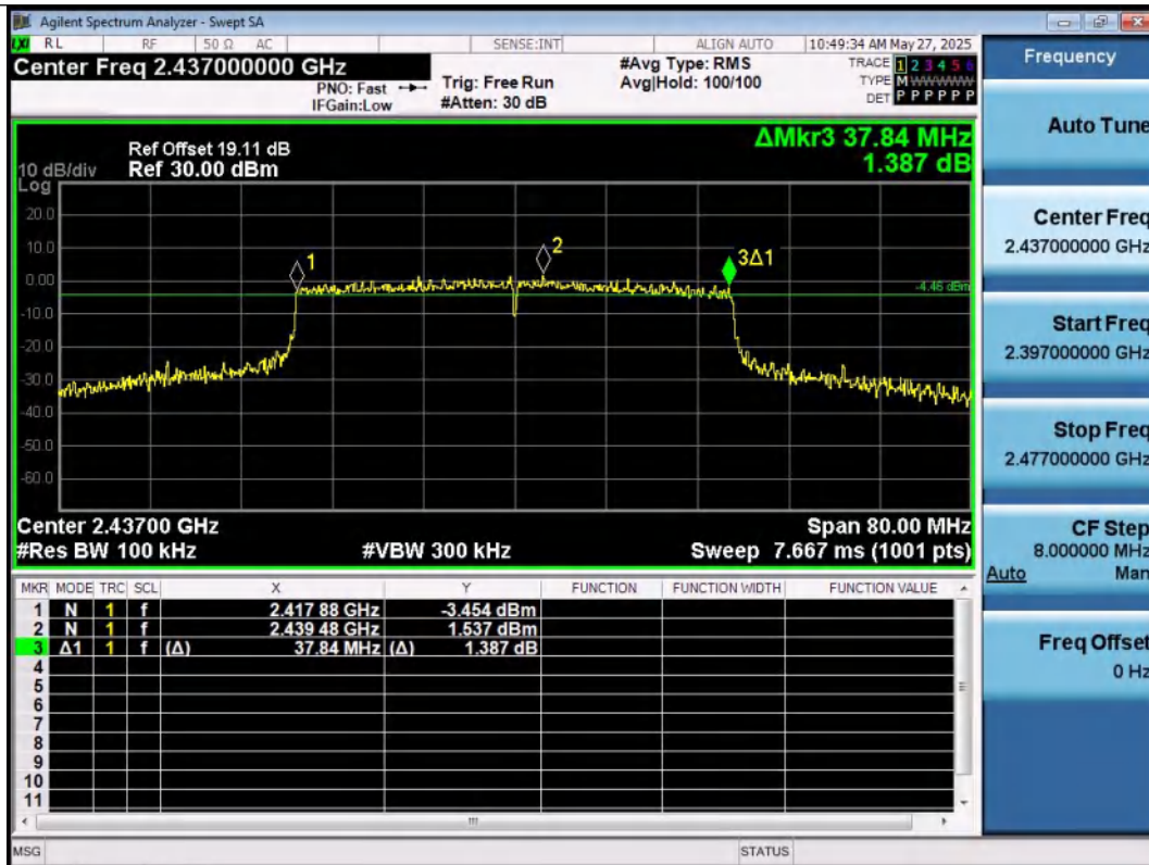
11AX40SISO-Ant1-2437-PASS
